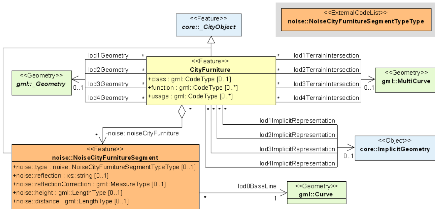
Figure H.8 – CityGML noise application schema – city furniture model (light yellow=CityGML CityFurniture module, light orange=CityGML Noise ADE). Prefixes are used to indicate XML namespaces associated with model elements. Element names without a prefix are defined within the CityGML CityFurniture module. The prefix noise is associated with the CityGML Noise ADE (source: Institute of Geodesy and Geoinformation Uni Bonn).
