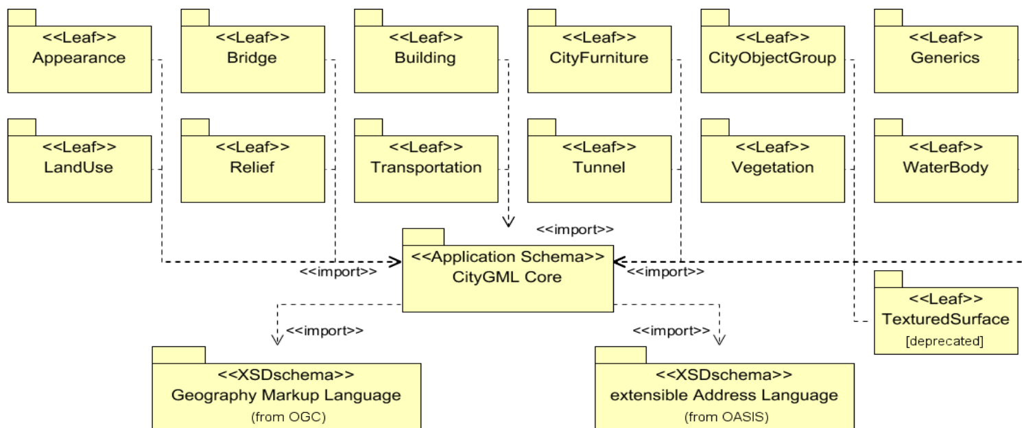
Figure 13 – UML package diagram illustrating the separate modules of CityGML and their schema dependencies. Each extension module (indicated by the leaf packages) further imports the GML 3.1.1 schema definition in order to represent spatial properties of its thematic classes. For readability reasons, the corresponding dependencies have been omitted.
