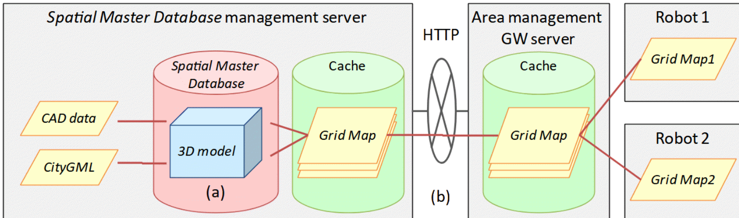
Figure I.3 – Configuration of a spatial master database management system.
