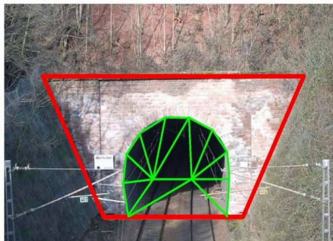
Figure 10-2 – TerrainIntersectionCurve for a tunnel object. The tunnel's hollow space is sealed by a triangulated ClosureSurface
