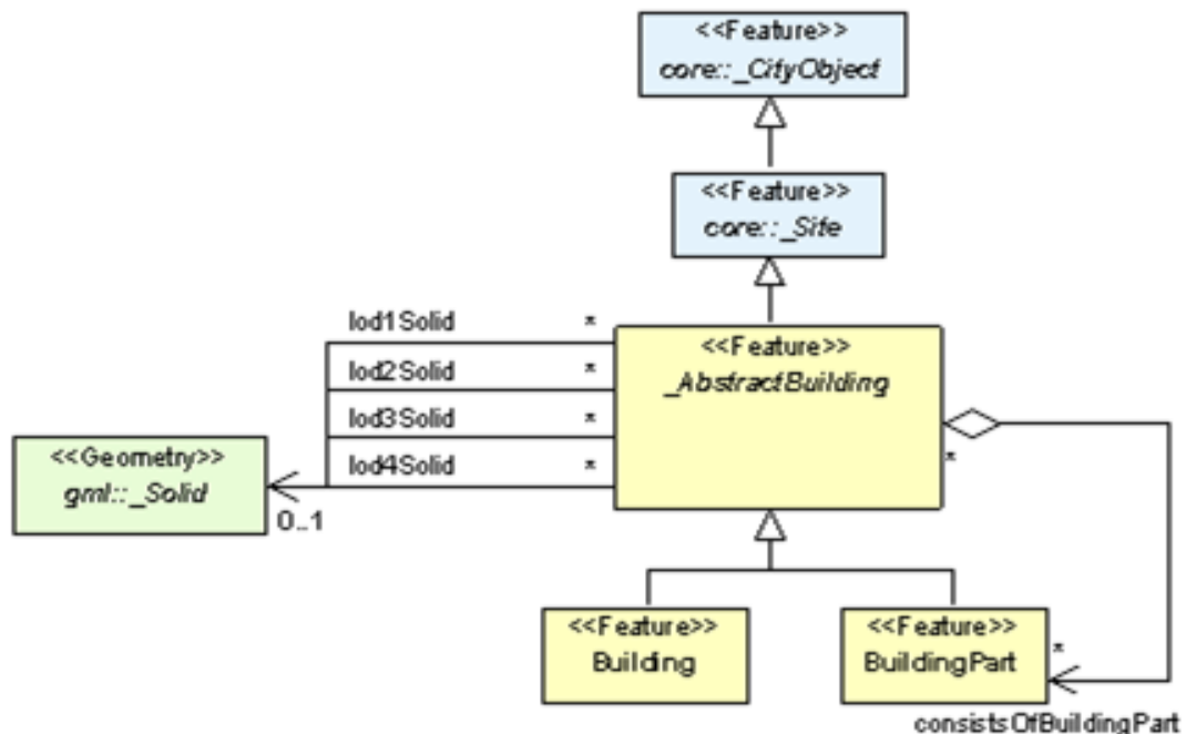
Figure 7 – Example UML diagram demonstrating the UML notation and coloring scheme used throughout the CityGML specification.
