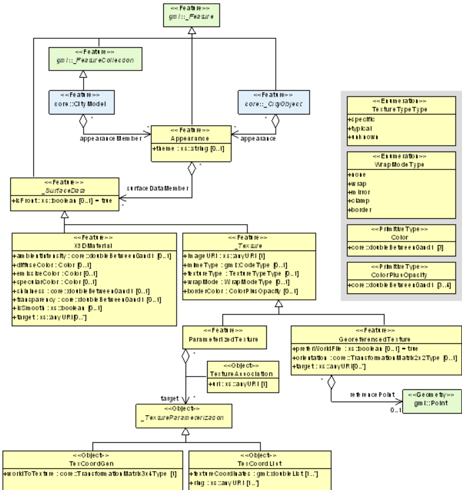
Figure 19 – UML diagram of CityGML's appearance model. Prefixes are used to indicate XML namespaces associated with model elements. Element names without a prefix are defined within the CityGML Appearance module.
