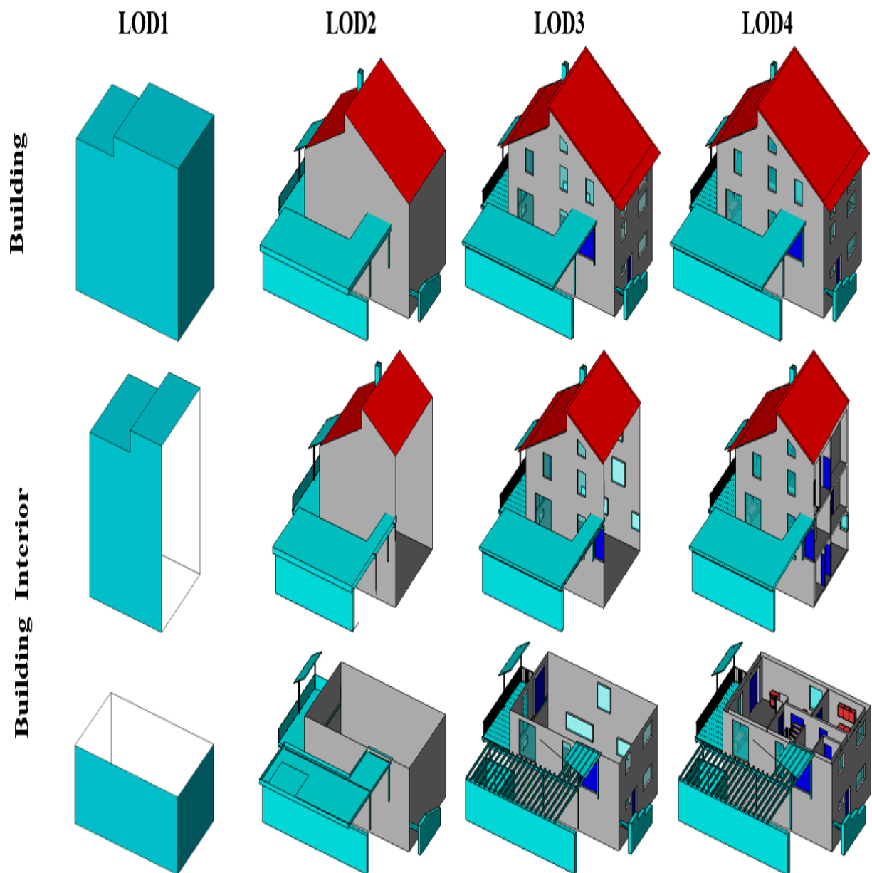
Figure 35 — Building model in LOD1 – LOD4 (source: Karlsruhe Institute of Technology (KIT), courtesy of Franz-Josef Kaiser).
