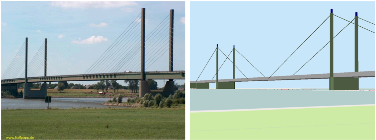
Figure 57 — The bridge of Rees (left photo (source: Harald Halfpapp); right LOD2 model (source: District of Recklinghausen / KIT)).
