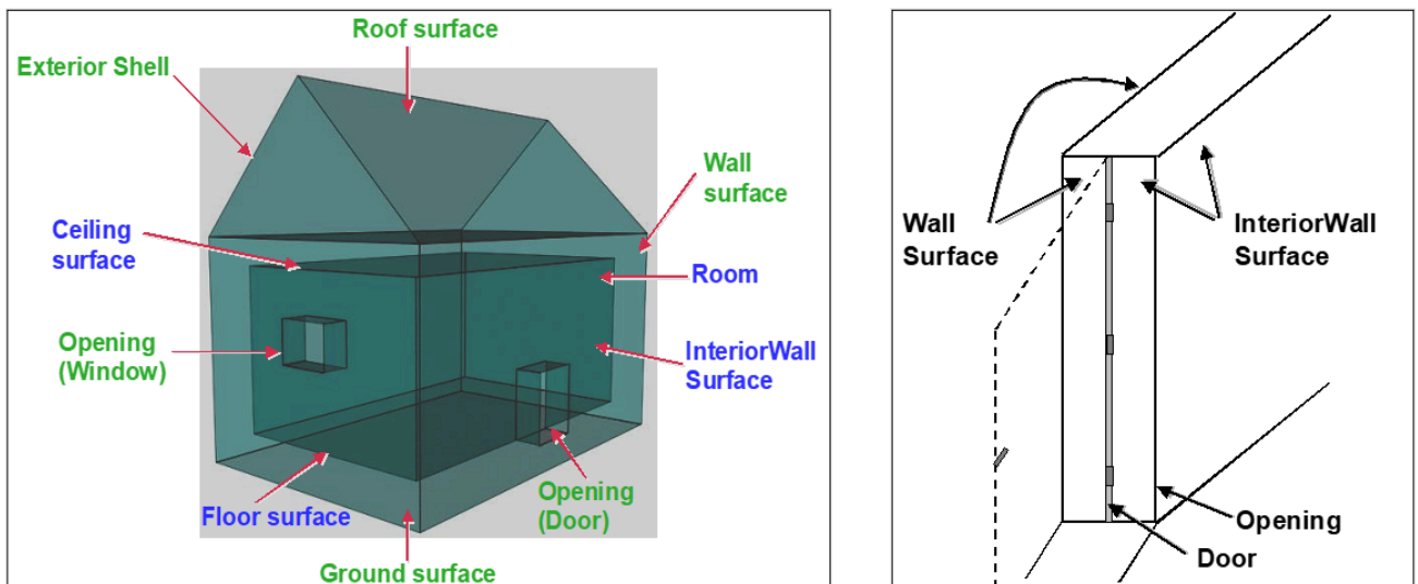
Figure 37 — Classification of BoundarySurfaces (left), in particular for Openings (right) (graphic: IGG Uni Bonn).
