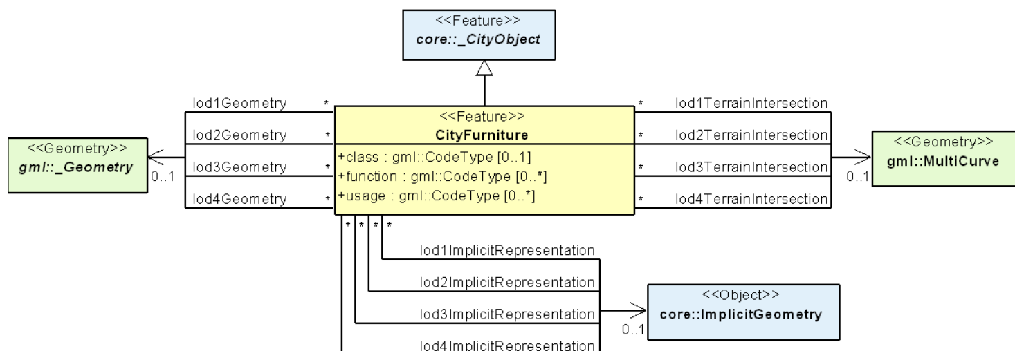
Figure 74 – UML diagram of city furniture objects in CityGML. Prefixes are used to indicate XML namespaces associated with model elements. Element names without a prefix are defined within the CityGML CityFurniture module.
