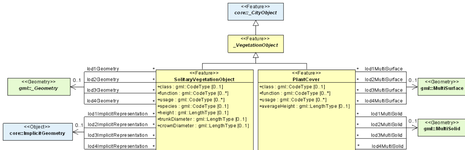
Figure 69 – UML diagram of vegetation objects in CityGML. Prefixes are used to indicate XML namespaces associated with model elements. Element names without a prefix are defined within the CityGML Vegetation module.
