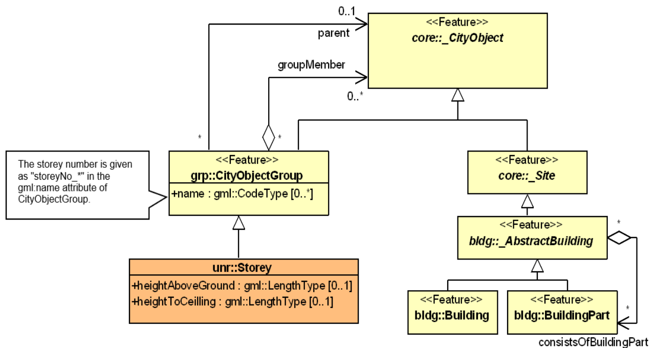
Figure I.7 – CityGML Robotics application schema – UNR Storey model (light yellow=CityGML module, light orange=UNR ADE). Prefixes are used to indicate XML namespaces associated with model elements. The prefix unr is associated with the UNR ADE (source: Central Research Laboratory, Hitachi, Ltd.). The CityGML model elements are associated with the recommended CityGML prefixes.
