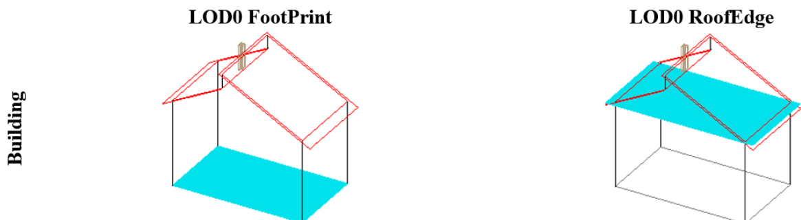
Figure 34 – The two possibilities of modeling a building in LOD0 using horizontal 3D surfaces. On the left, the building footprint ( lod0FootPrint ) is shown (cyan) which denotes the shape of the building on the ground. The corresponding surface representation is located at ground level. On the right, the lod0RoofEdge representation is illustrated (cyan) which
