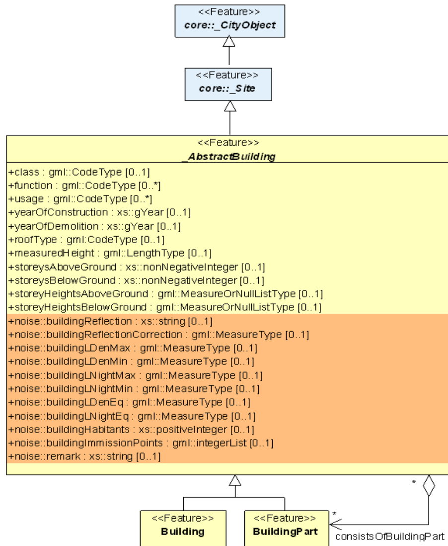
Figure H.7 – CityGML noise application schema – excerpt of the building model (light yellow=CityGML Building module, light orange=CityGML Noise ADE). Prefixes are used to indicate XML namespaces associated with model elements. Element names without a prefix are defined within the CityGML Building module. The prefix noise is associated with the CityGML Noise ADE (source: Institute of Geodesy and Geoinformation Uni Bonn).
