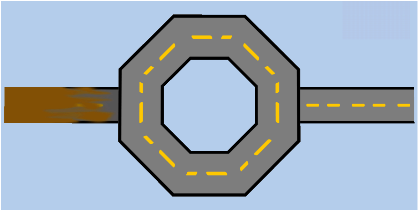
Figure G.15 — A rendering of the textured geometry (images for this example: Hasso-Plattner-Institute).
