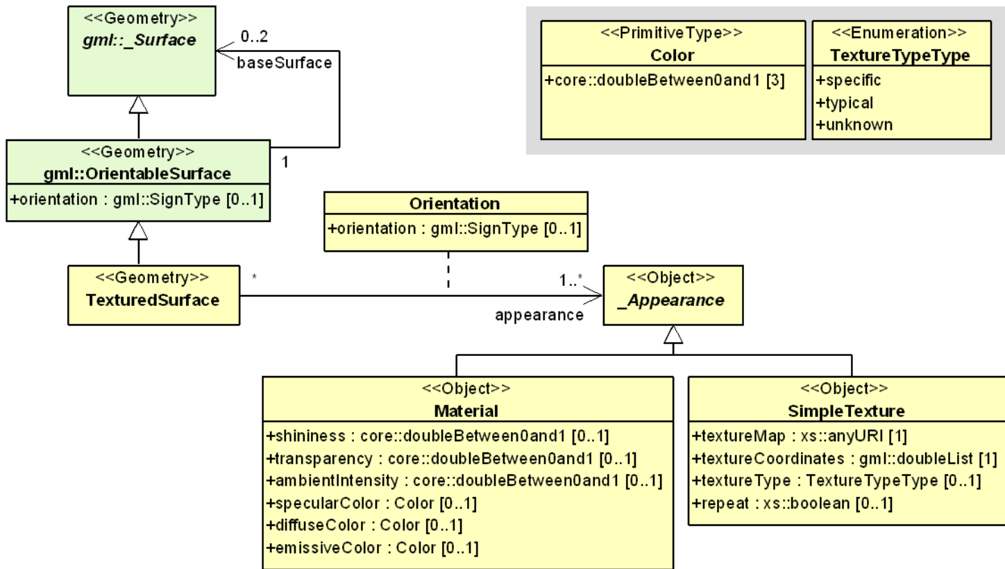
Figure 25 – UML diagram of CityGML's material model. Please note, that this approach for appearance modelling has been marked as deprecated and is expected to be removed in future CityGML versions. Prefixes are used to indicate XML namespaces associated with model elements. Element names without a prefix are defined within the CityGML TexturedSurface module.
