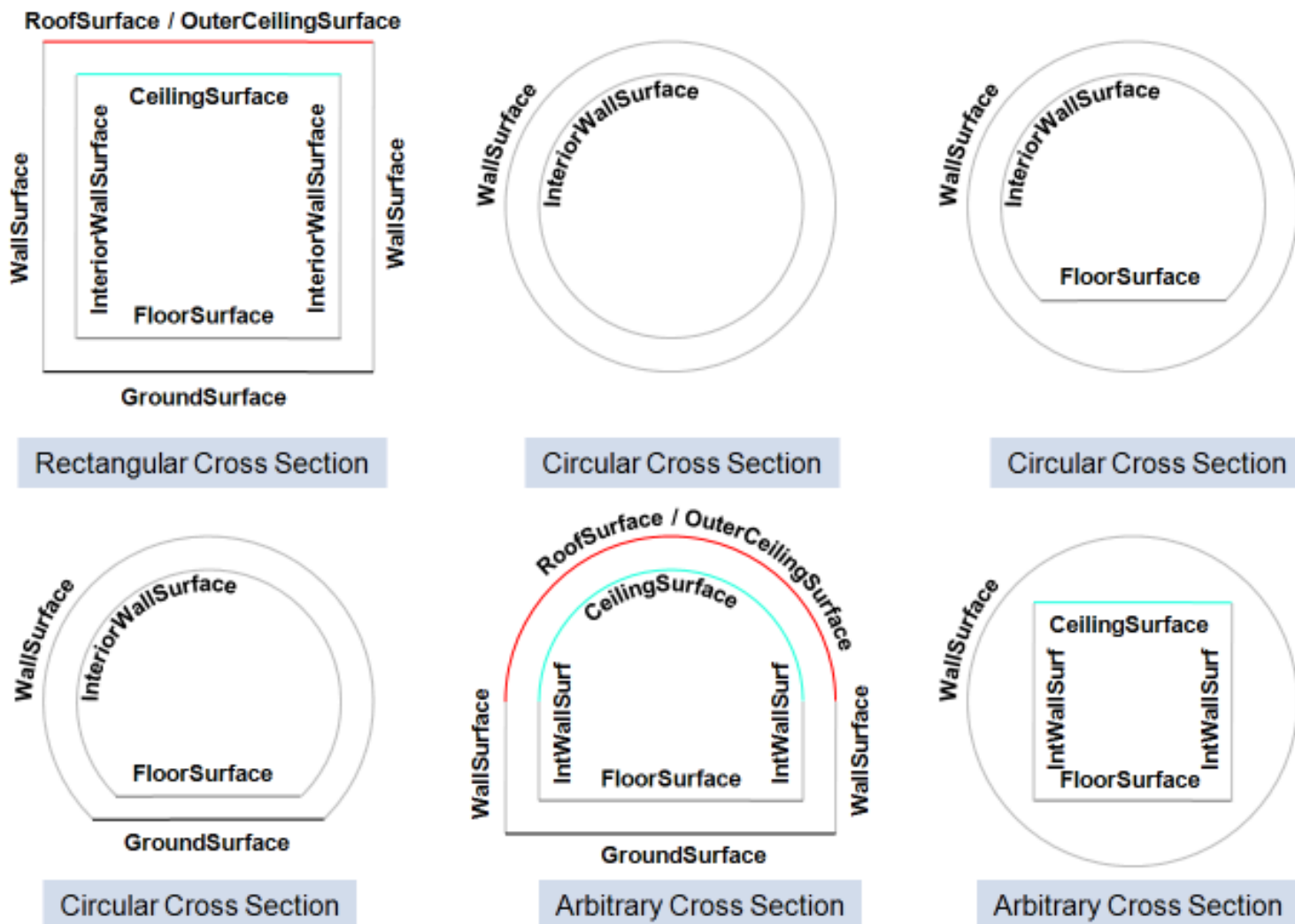
Figure 46 – Examples for the use of boundary surfaces for tunnels with different cross sections. WallSurface , RoofSurface , GroundSurface , OuterCeilingSurface and OuterFloorSurface are available in LOD2 - 4, whereas InteriorWallSurface , FloorSurface and CeilingSurface may only be used in LOD4 to model the interior boundary surfaces of a hollow space.
