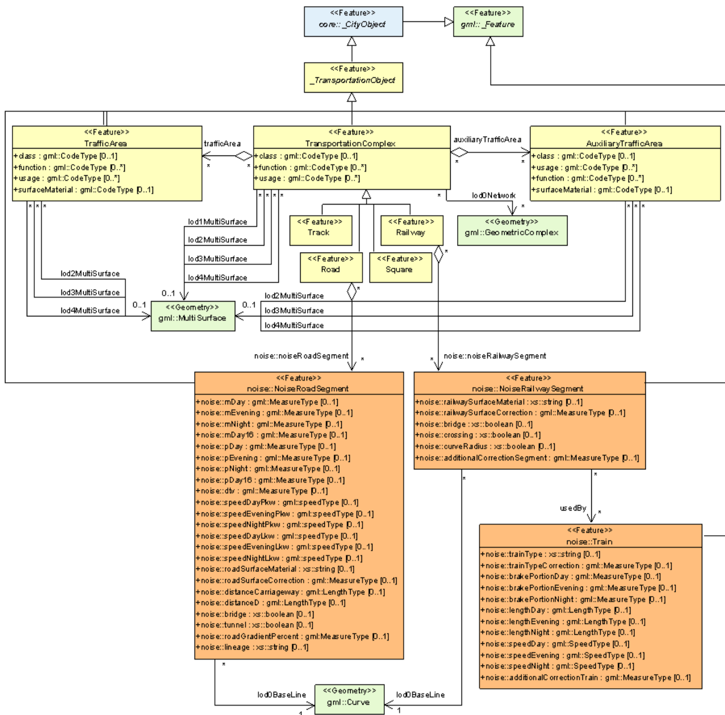
Figure H.6 – CityGML noise application schema – transportation model (light yellow=CityGML Transportation module, light orange=CityGML Noise ADE). Prefixes are used to indicate XML namespaces associated with model elements. Element names without a prefix are defined within the CityGML Transportation module. The prefix noise is associated with the CityGML Noise ADE (source: Institute of Geodesy and Geoinformation Uni Bonn).
