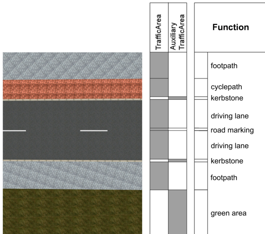
Figure 66 – TransportationComplex in LOD 2-4: representation of a road with a complex cross-section profile (example shows urban road) (source: Rheinmetall Defence Electronics).
