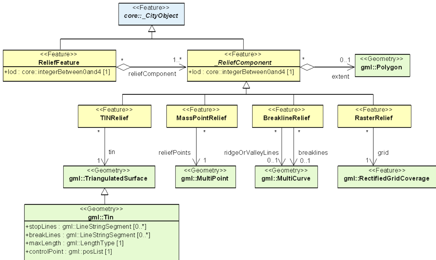
Figure 29 – UML diagram of the Digital Terrain Model in CityGML. Prefixes are used to indicate XML namespaces associated with model elements. Element names without a prefix are defined within the CityGML Relief module.
