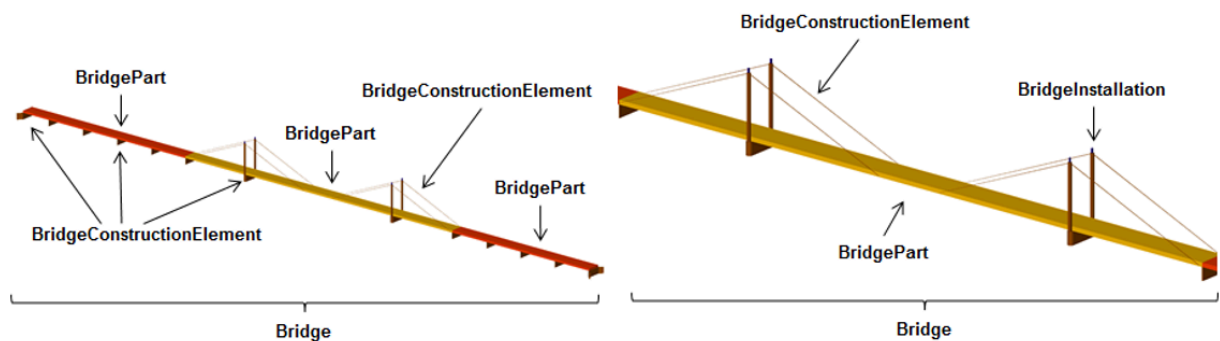
Figure 56 – The bridge of Rees, consisting of a Bridge feature and three BridgePart features (left). The bridge contains BridgeConstructionElement and BridgeInstallation features (right).
