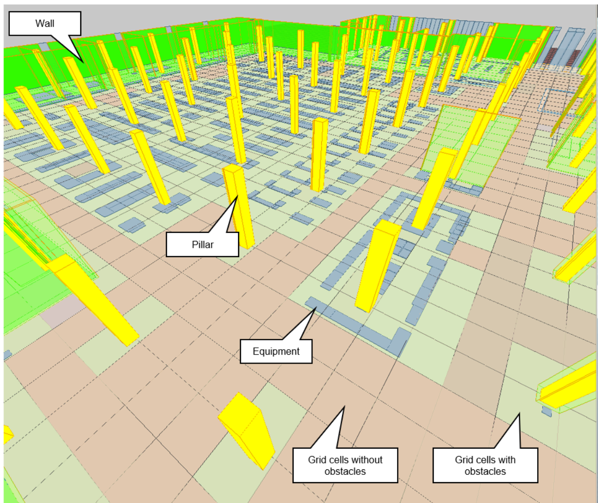
Figure I.1 — 3D spatial master database for a shopping mall. This was generated from CityGML with Robotics ADE and used for the ubiquitous network robots services research project in Japan. The height of each floor is set up when turning the original 2D CAD data into 3D data in the spatial master database. Thus, the heights of some equipment (for example, furniture) is not set up and is displayed in 2D. Also, the grid map (with obstacles information) generated by the grid map function of the spatial master database is attached to the ground on the floor surface. The grid map consists of grid cells of a given size, and is color-coded depending on whether obstacles exist or not. Robots use these grid maps to recognize whether they can pass through each grid (green=walls, yellow=pillars, blue=equipment, green floor=grid cells with obstacles such as pillars and furniture, red floor=grid cells without obstacles).
