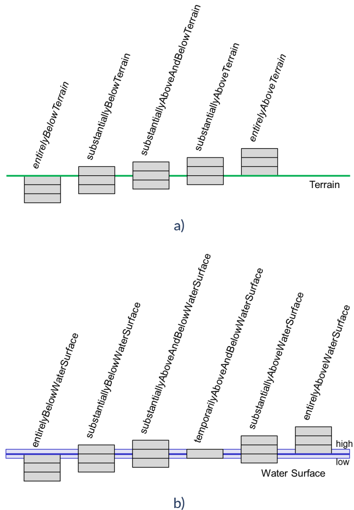
Figure 27 – Topological relations of a CityGML object with respect to a) the terrain and b) the water surface.
