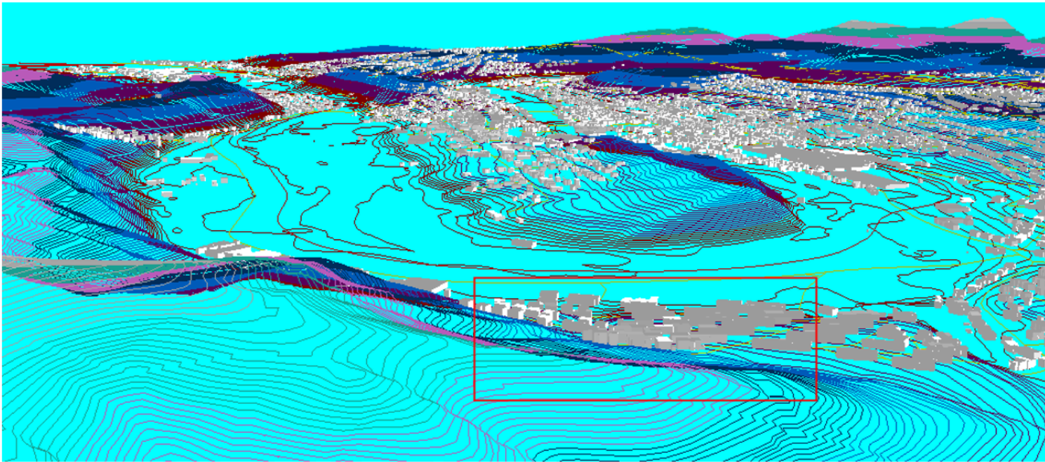
Figure H.4 – 3D geodata in CityGML for the calculation of the noise map in Figure H.1: Derived contour lines for the generation of CityGML breaklines, 3D block model in CityGML, 3D road and railway data in CityGML, state road data for higher-level roads in CityGML (source: Surveying and Mapping Agency NRW, State Road Enterprise NRW, Stapelfeldt GmbH, Institute of Geodesy and Geoinformation Uni Bonn).
