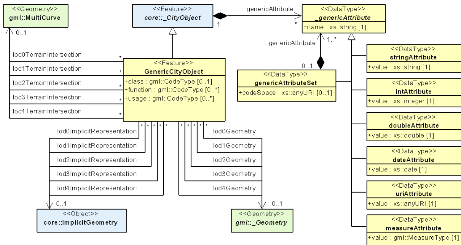
Figure 79 – UML diagram of generic objects and attributes in CityGML. Prefixes are used to indicate XML namespaces associated with model elements. Element names without a prefix are defined within the CityGML Generics module.
