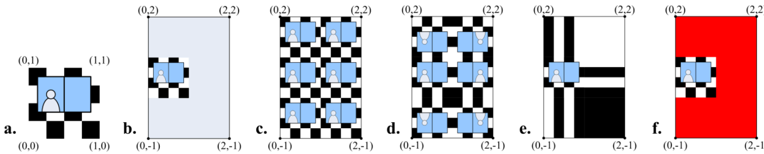
Figure 20 — A texture (a) applied to a facade using different wrap modes: (b) none, (c) wrap, (d) mirror, (e) clamp and (f) border. The border color is red. The numbers denote texture coordinates (image: Hasso-Plattner-Institute).
