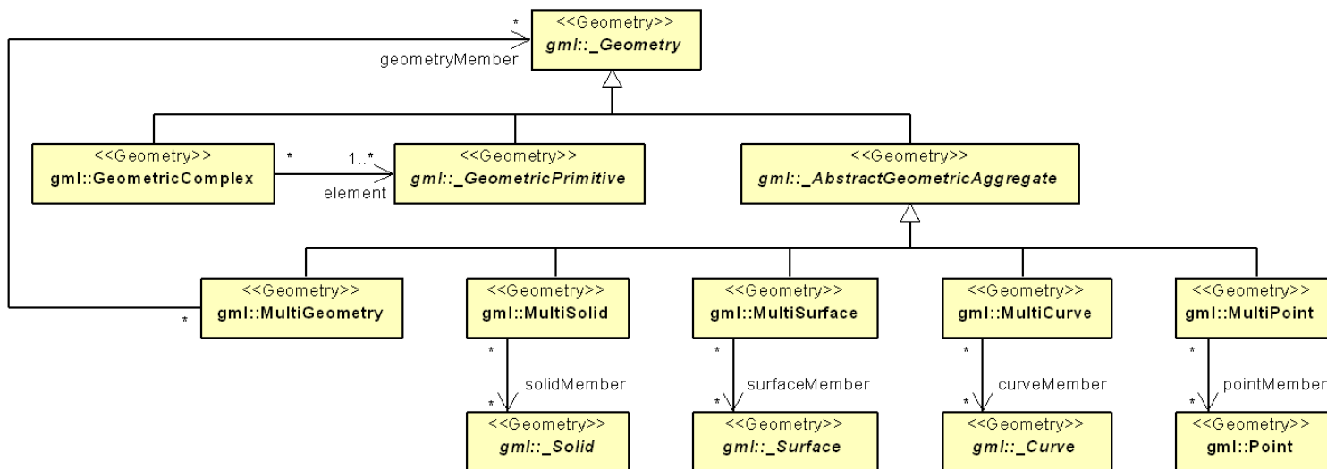
Figure 15 – UML diagram of CityGML's geometry model: Complexes and Aggregates
