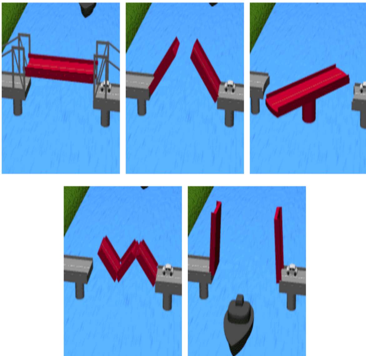
Figure 52 — Examples for movable bridges (source: ISO 6707).
