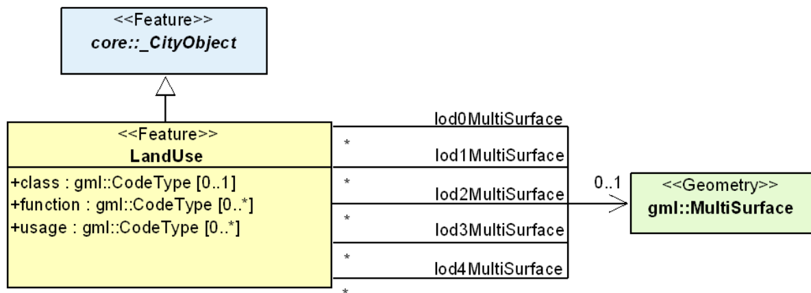
Figure 76 – UML diagram of land use objects in CityGML. Prefixes are used to indicate XML namespaces associated with model elements. Element names without a prefix are defined within the CityGML LandUse module.
