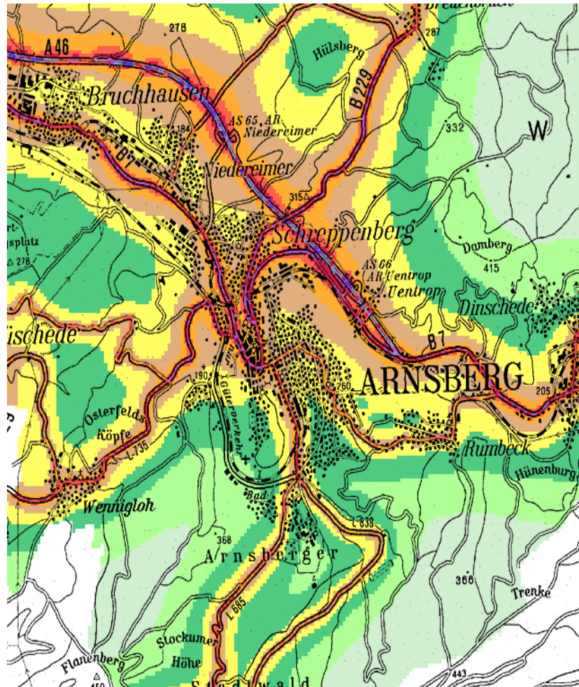
Figure H.1 — Noise map generated from the 3D CityGML geodata and used for the reporting demanded of the EU Environmental Noise Directive (dark colours show higher noise immission) (source: State Agency for nature, environment and consumer protection NRW).
