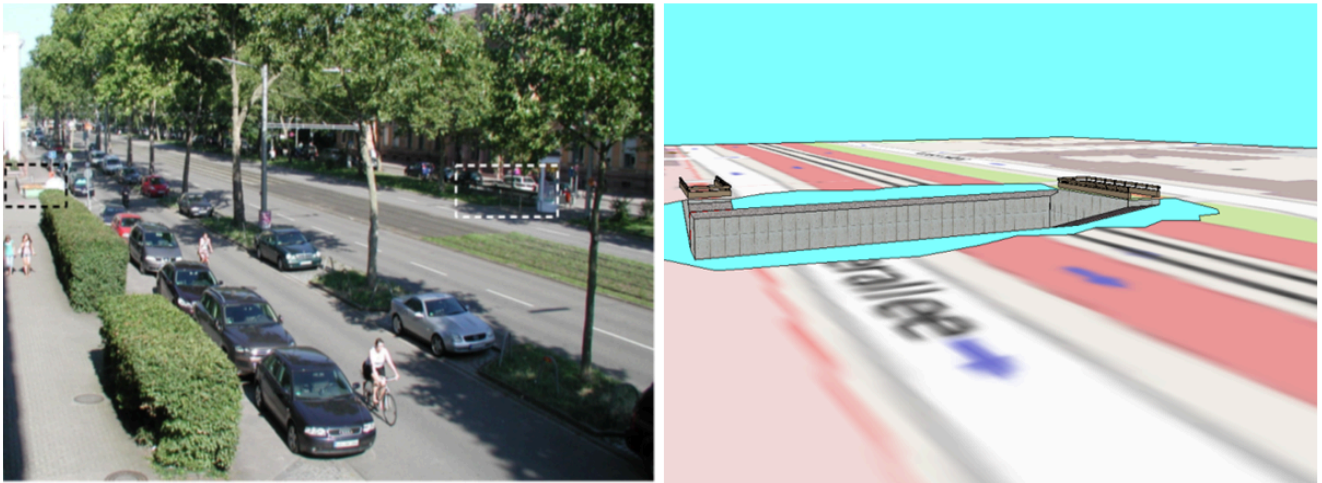
Figure 47 — Example of a tunnel modeled in LOD3 (real situation on the left side; CityGML model on the right side) (source: Karlsruhe Institute of Technology (KIT), courtesy of City of Karlsruhe).
