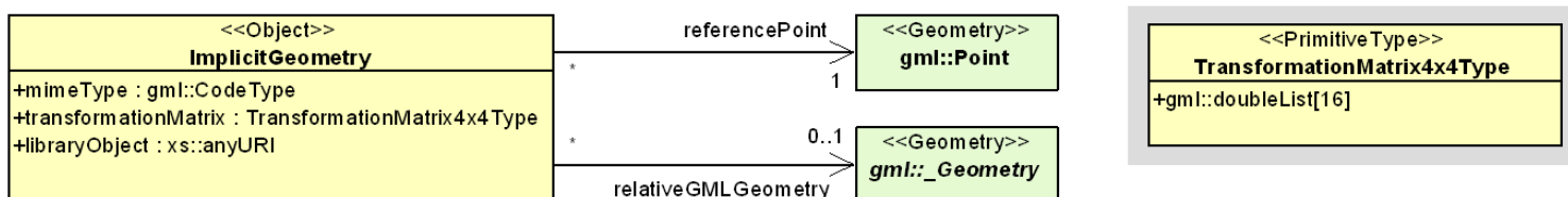
Figure 18 – UML diagram of ImplicitGeometries . Prefixes are used to indicate XML namespaces associated with model elements. Element names without a prefix are defined within the CityGML Core module.
