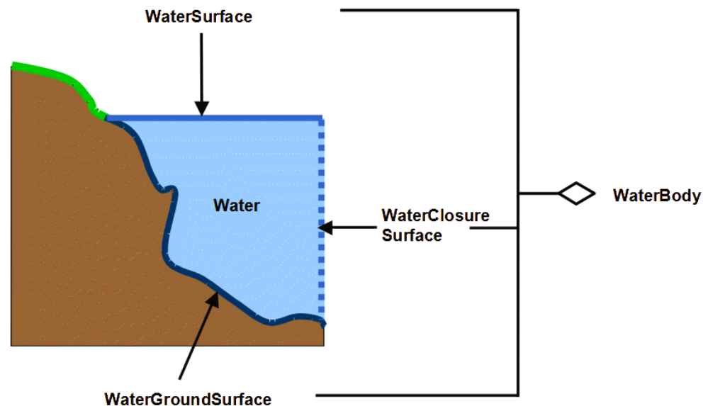
Figure 60 — Illustration of a water body defined in CityGML (graphic: IGG Uni Bonn).
