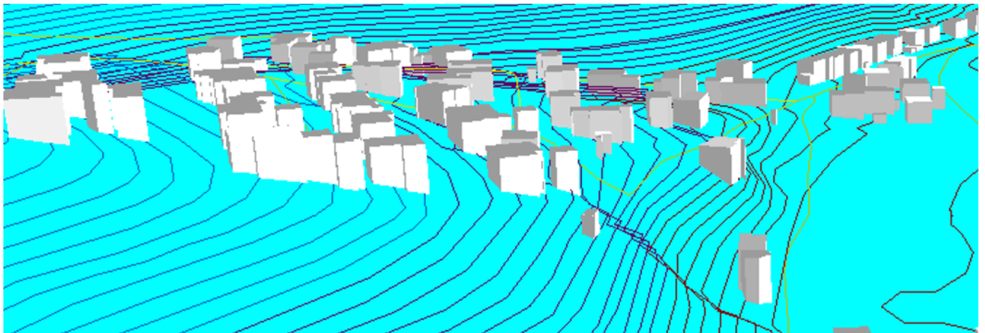
Figure H.5 – Extract from Figure H.4 shows the integration of 3D block models in the DTM by appropriate CityGML modelling (lowest point of ALK building polygon is taken as measure to generate the building bottom side) (source: Surveying and Mapping Agency NRW, Stapelfeldt GmbH, Institute of Geodesy and Geoinformation Uni Bonn).
