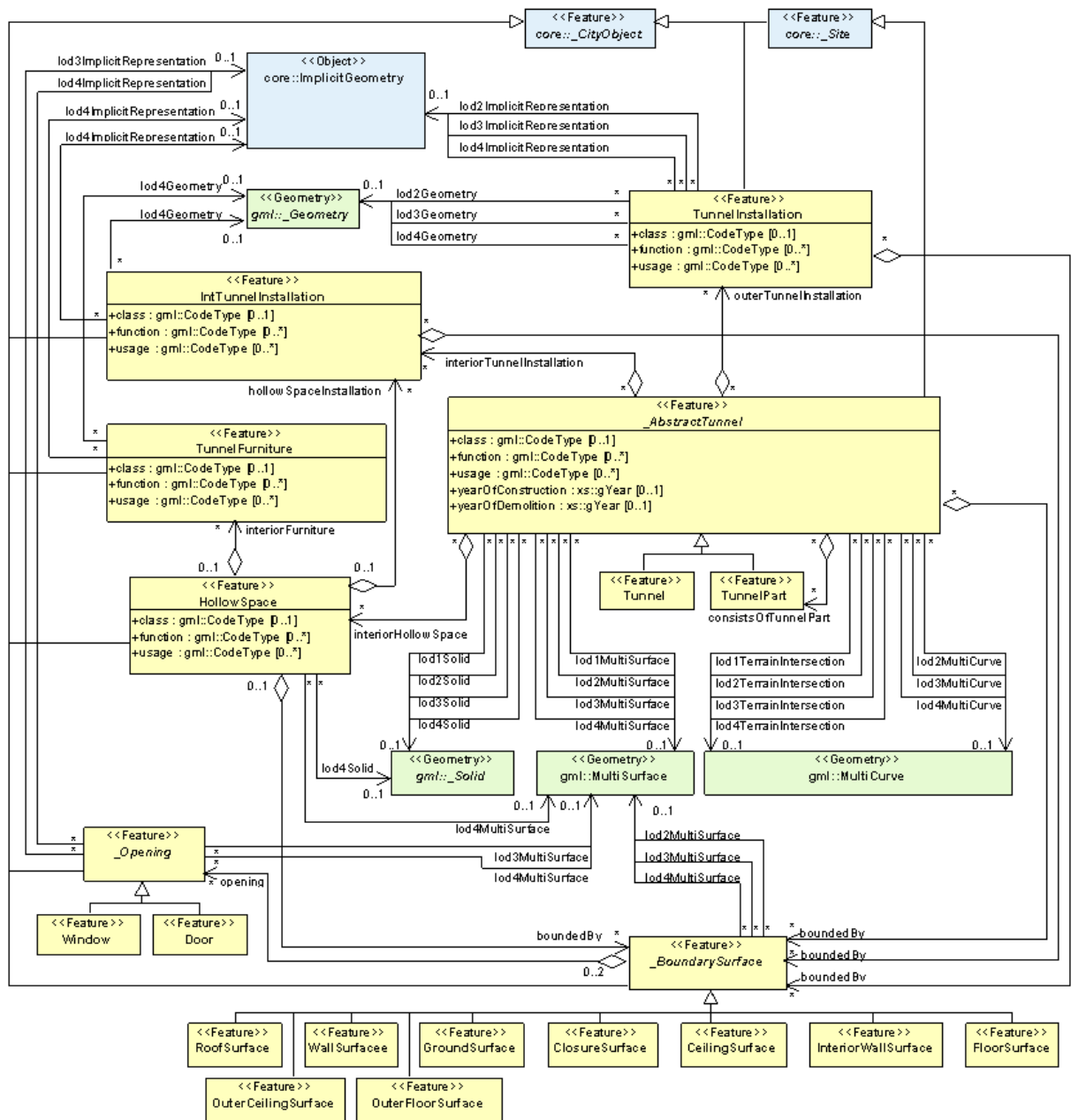
Figure 43 — UML diagram of CityGML's tunnel model. Prefixes are used to indicate XML namespaces associated with model elements. Element names without a prefix are defined within the CityGML Tunnel module.
