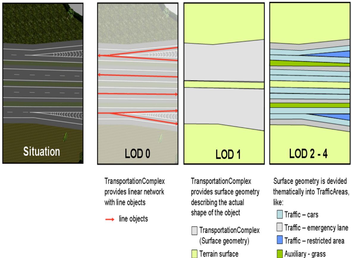
Figure 65 – TransportationComplex in LOD0, 1, and 2-4 (example shows part of a motorway) (source: Rheinmetall Defence Electronics).
