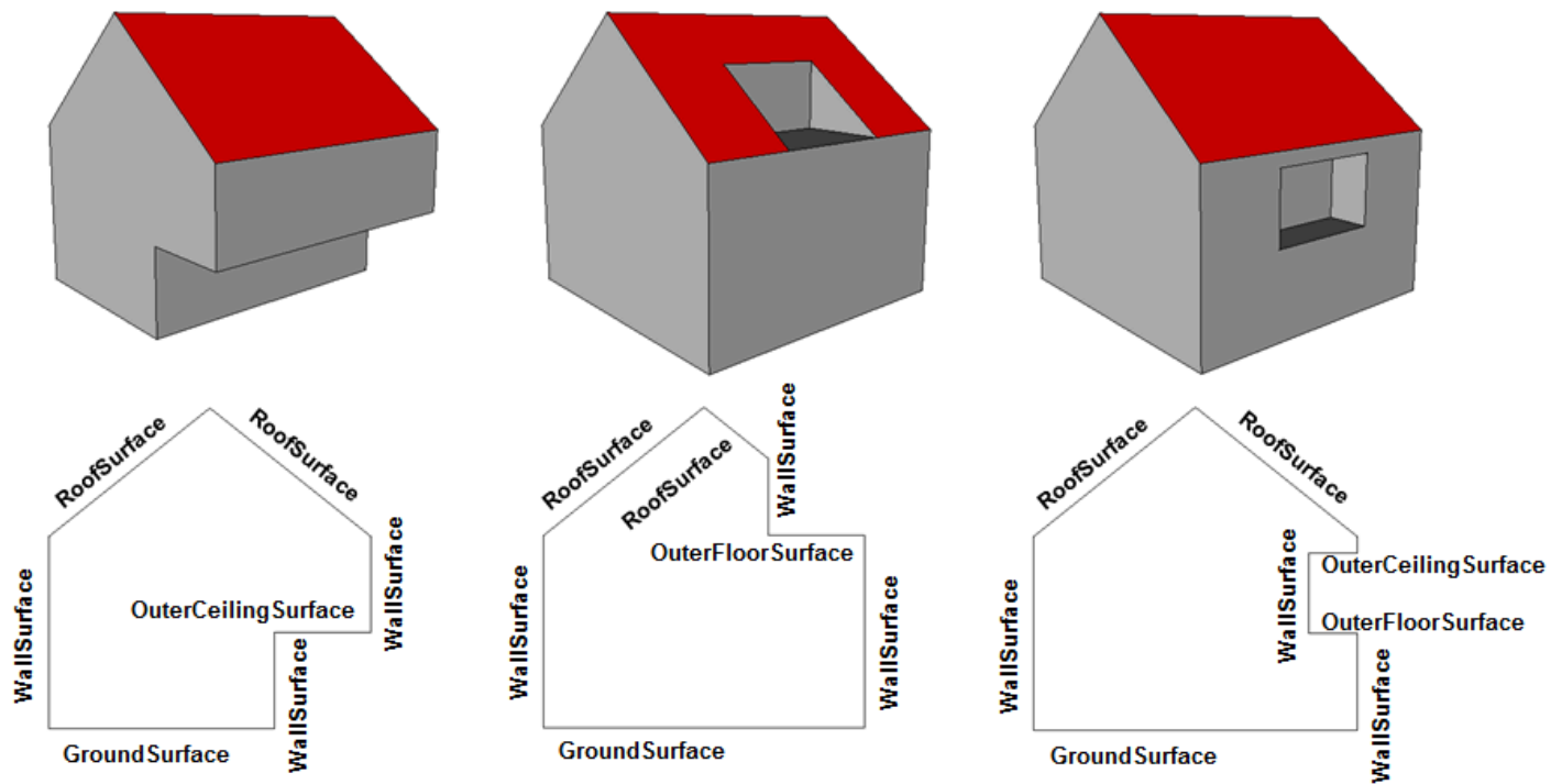
Figure 36 – Examples of the classification of _BoundarySurfaces of the outer building shell (source: Karlsruhe Institute of Technology (KIT))
