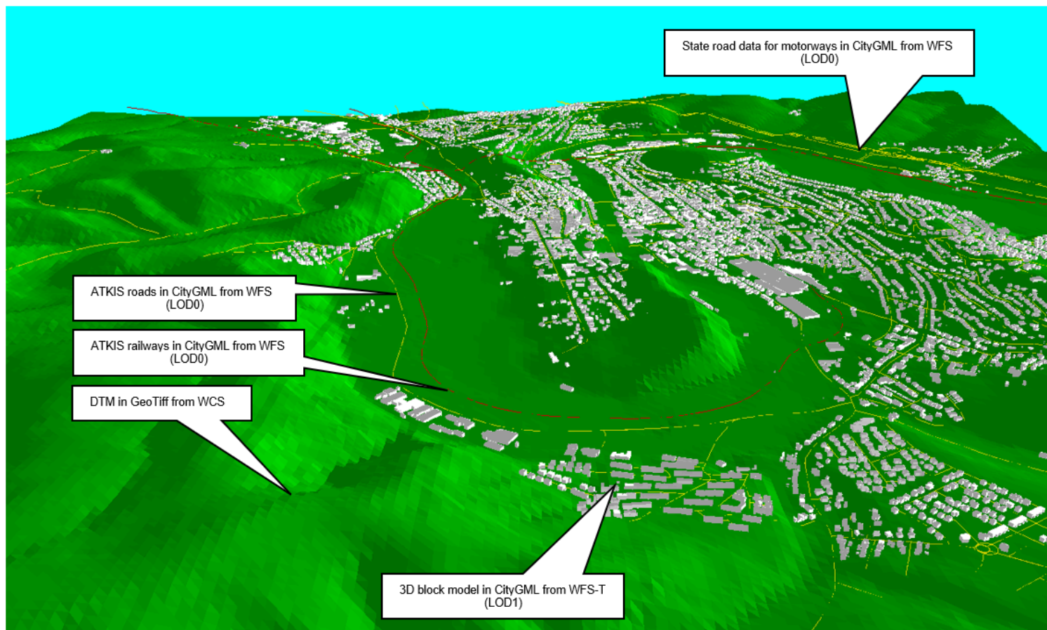
Figure H.3 — 3D geodata in CityGML for the calculation of the noise map in Figure H.1: DTM in GeoTiff, 3D block model in CityGML, 3D road and railway data in CityGML, state road data for higher-level roads in CityGML (source: Surveying and Mapping Agency NRW, State Road Enterprise NRW, Stapelfeldt GmbH, Institute of Geodesy and Geoinformation Uni Bonn).
