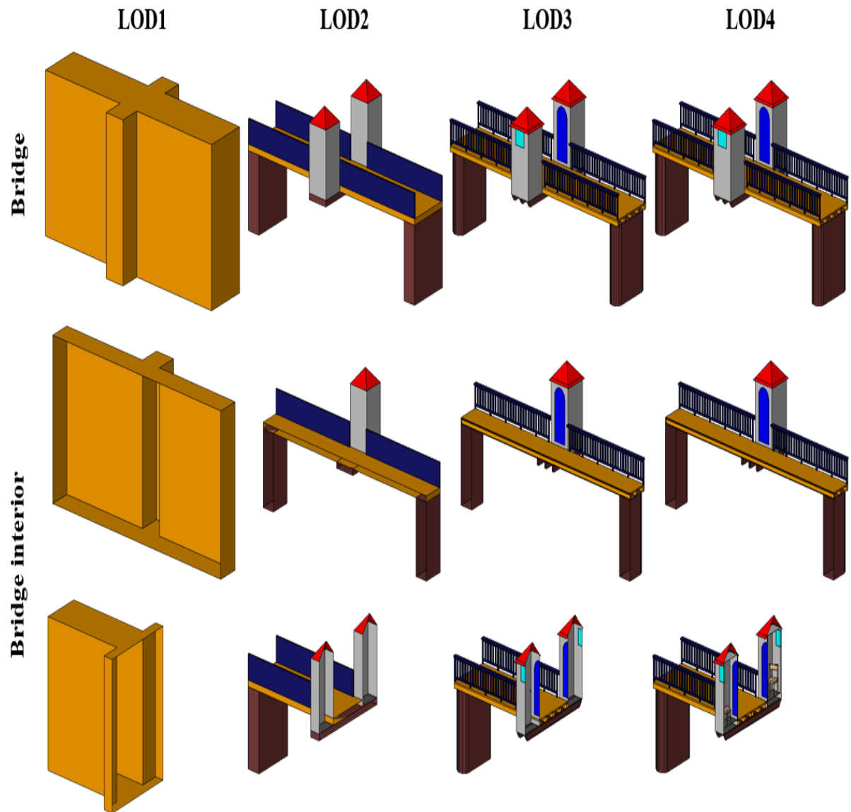
Figure 51 — Bridge model in LOD1 – LOD4. (source: Karlsruhe Institute of Technology (KIT))
