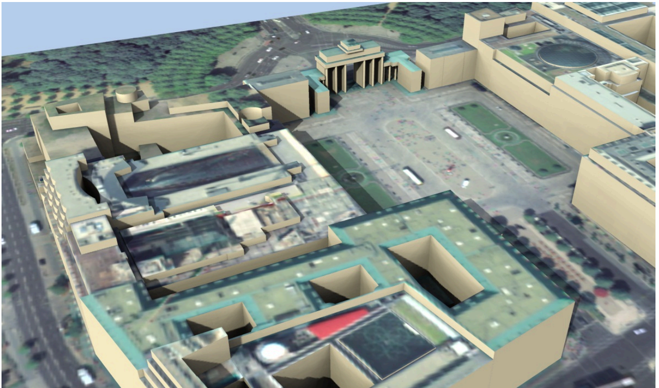
Figure 21 — A georeferenced texture applied to ground and roof surfaces (source: Senate of Berlin, Hasso-Plattner-Institute).
