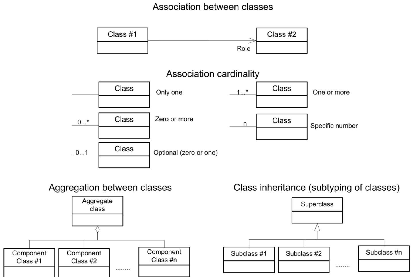
Figure 6 – UML notation (see ISO TS 19103, Geographic information - Conceptual schema language).
