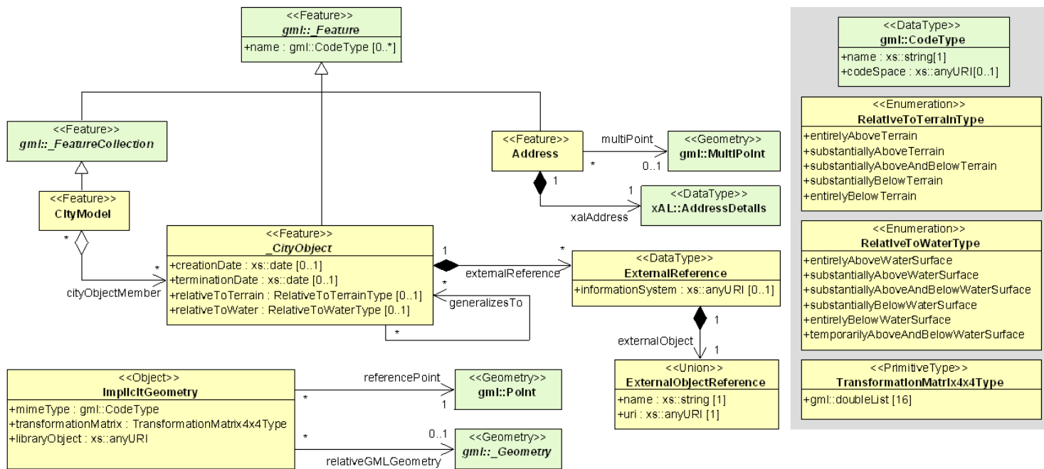
Figure 26 – UML diagram of CityGML's core module. The bracketed numbers following the attribute names denote the attribute's multiplicity: the minimal and maximal number of occurrences of the attribute per object. For example, a name is optional (0) in the class _Feature or may occur multiple times (star symbol), while a _CityObject has none or at most one creationDate . Prefixes are used to indicate XML namespaces associated with model elements. Element names without a prefix are defined within the CityGML Core module.
