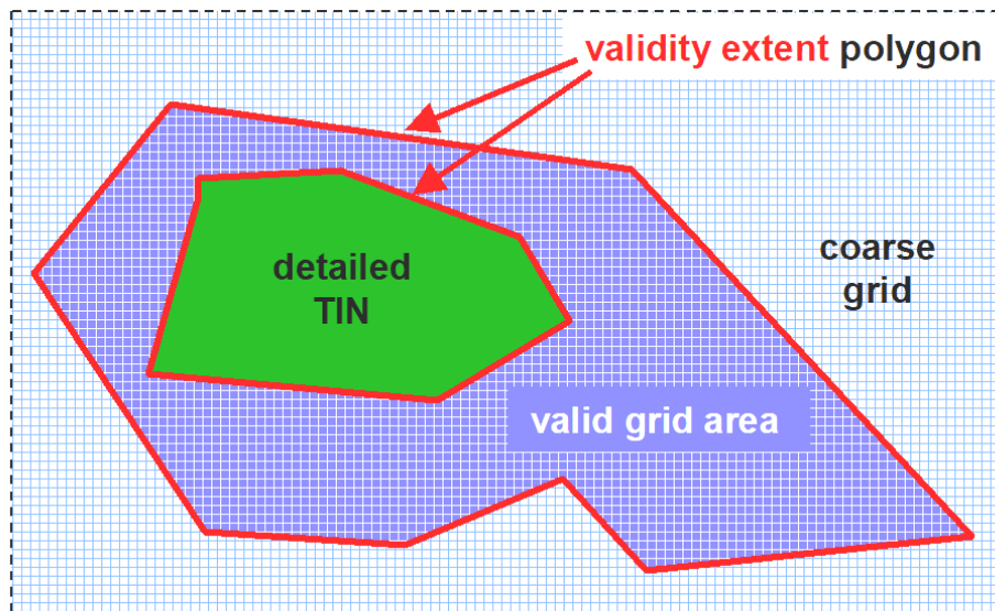
Figure 30 – Nested DTMs in CityGML using validity extent polygons (graphic: IGG Uni Bonn).
