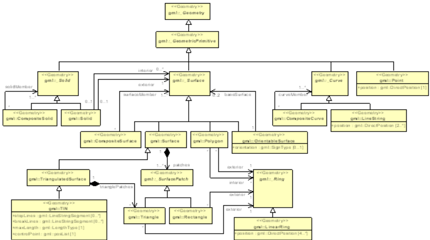
Figure 14 – UML diagram of CityGML's geometry model (subset and profile of GML3): Primitives and Composites.
