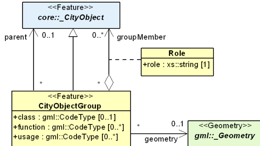
Figure 78 – UML diagram of city object groups in CityGML. Prefixes are used to indicate XML namespaces associated with model elements. Element names without a prefix are defined within the CityGML CityObjectGroup module.
