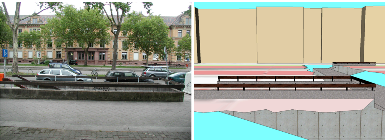
Figure 48 — The same LOD3 tunnel shown from a different perspective. The camera is positioned in front of the left entrance and pointing in the direction of the right entrance. (real situation on the left side; CityGML model on the right side). The model on the right also includes an LOD1 representation of the nearby buildings in the background (painted in light brown) (source: Karlsruhe Institute of Technology (KIT), courtesy of City of Karlsruhe).
