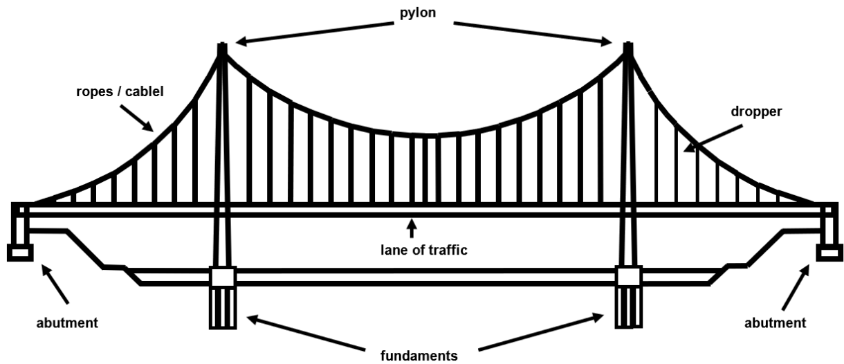
Figure 54 – BridgeConstructionElements of a suspension bridge.
