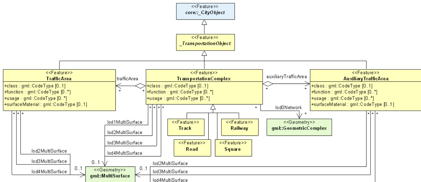
Figure 64 – UML diagram of the transportation model in CityGML. Prefixes are used to indicate XML namespaces associated with model elements. Element names without a prefix are defined within the CityGML Transportation module.
