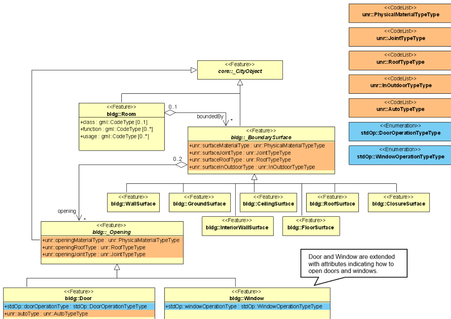
Figure I.6 – CityGML Robotics application schema – Standard Openings and UNR models including Door and Window (light yellow=CityGML modules, light blue=CityGML Standard Opening ADE, light orange=UNR ADE). Prefixes are used to indicate XML namespaces associated with model elements. The prefix stdOp is associated with the CityGML Standard Opening ADE (source: Institute for Geodesy and Geoinformation Science, Technical University Berlin), and the prefix unr is associated with the UNR ADE (source: Central Research Laboratory, Hitachi, Ltd.). The CityGML model elements are associated with the recommended CityGML prefixes.
