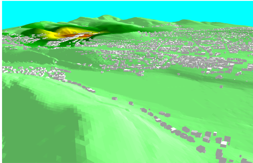
Figure H.2 – Modelling a noise emission source using the 3D CityGML geodata in a special noise calculation software as first step before generating the noise map in Figure H.1 (source: Surveying and Mapping Agency NRW, Stapelfeldt GmbH, Institute of Geodesy and Geoinformation Uni Bonn).
