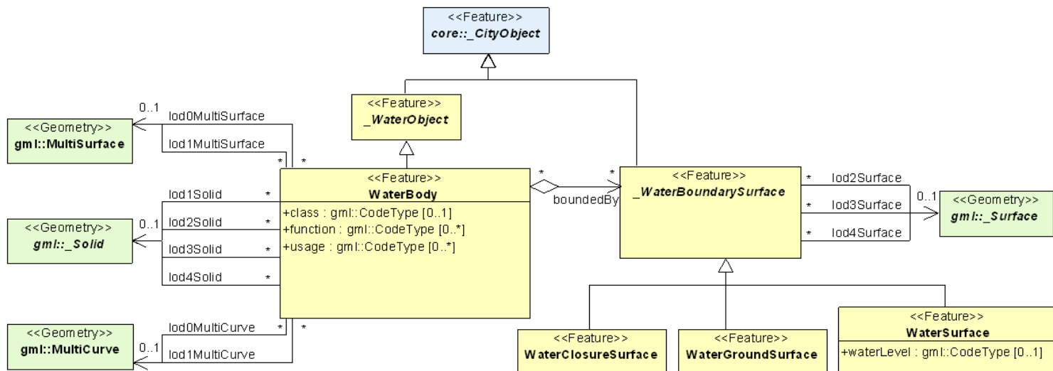
Figure 61 – UML diagram of the water body model in CityGML. Prefixes are used to indicate XML namespaces associated with model elements. Element names without a prefix are defined within the CityGML WaterBody module.
