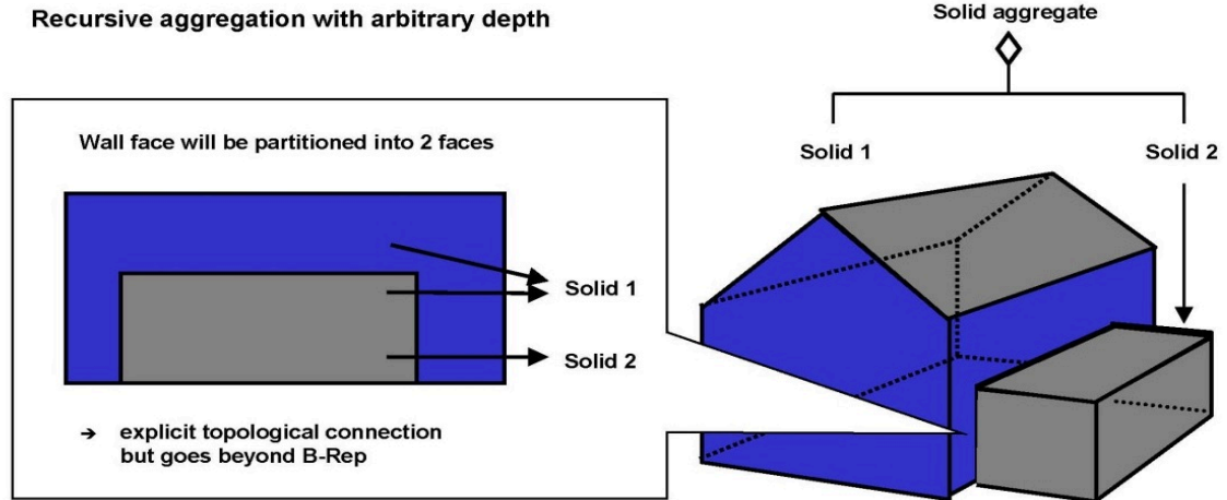
Figure 17 – Recursive aggregation of objects and geometries in CityGML (graphic: IGG Uni Bonn).
