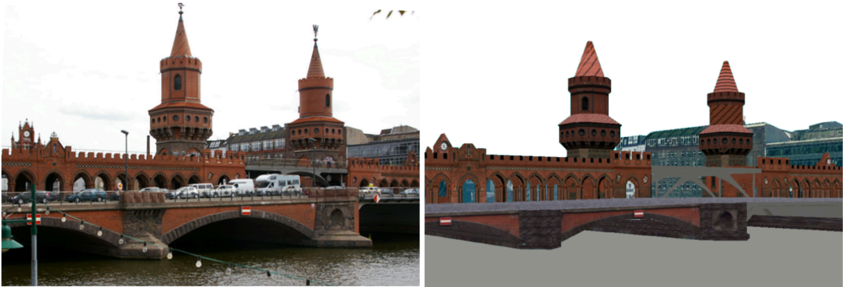
Figure 59 – The bridge "Oberbaumbrücke" in Berlin represented as bridge model in LOD4 (left a photo, right the 3D CityGML model) (source: Berlin Senate of Business, Technology and Women; Business Location Center, Berlin; Technische Universität Berlin; Karlsruhe Institute of Technology (KIT)).
