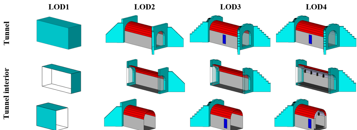
Figure 45 — Tunnel model in LOD1 – LOD4 (source: Karlsruhe Institute of Technology (KIT)).
