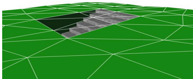
Figure 9-2 — The entrance is sealed by a virtual ClosureSurface , which is both part of the DTM and the subsurface object
