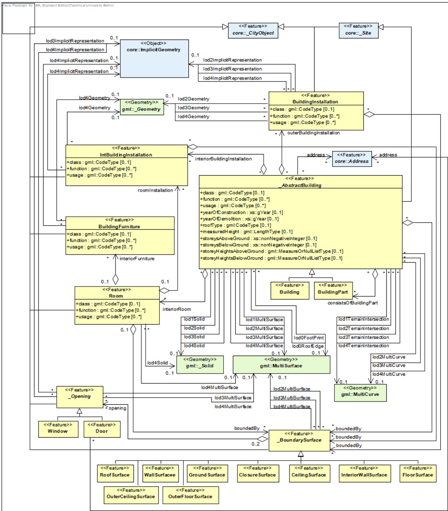
Figure 32 – UML diagram of CityGML's building model. Prefixes are used to indicate XML namespaces associated with model elements. Element names without a prefix are defined within the CityGML Building module.
