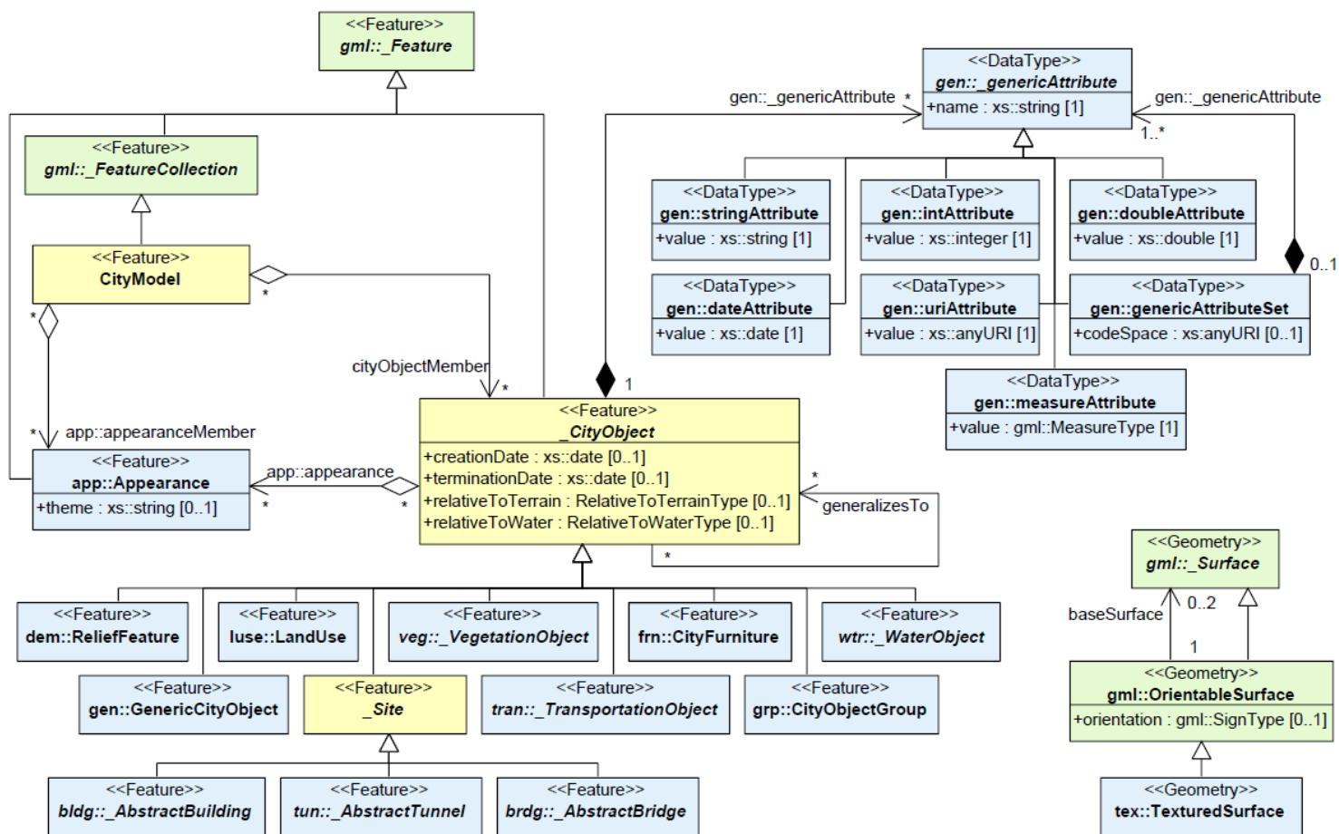
Figure 28 – CityGML's top level class hierarchy. Prefixes are used to indicate XML namespaces associated with model elements. Element names without a prefix are defined within the CityGML Core module.
