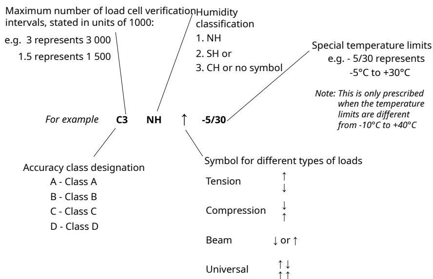
Figure 4 — Complete load cell classification
