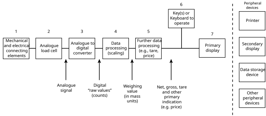
From OIML R 76: Definition of typical modules within a weighing system (other combinations are possible).
