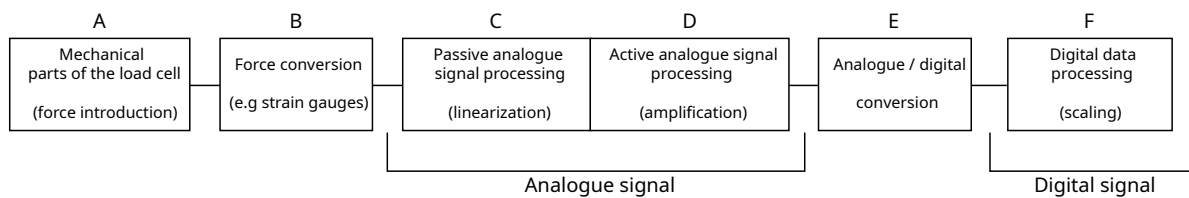
Figure 1 — Typical components in a weighing instrument
