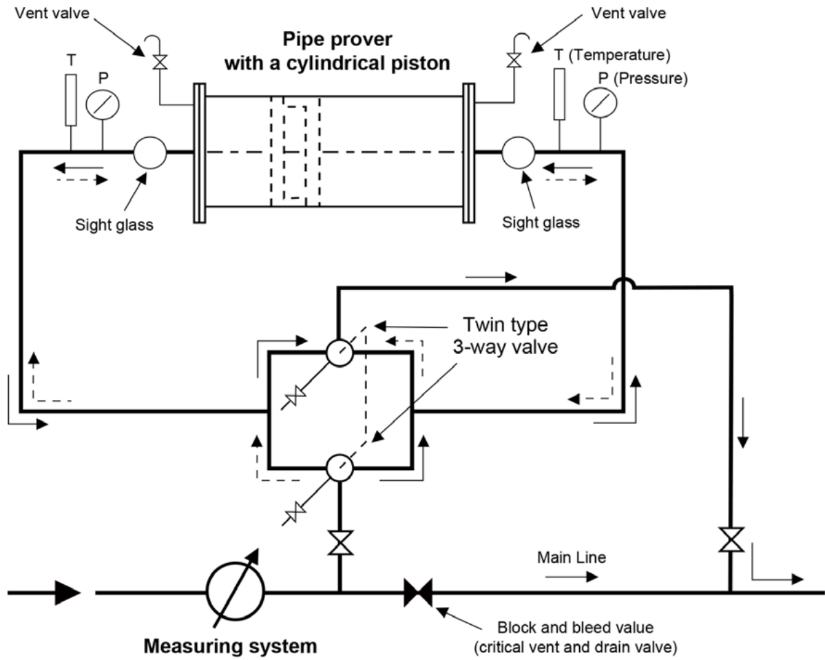
Figure A.6 — Typical full stroke type pipe prover
