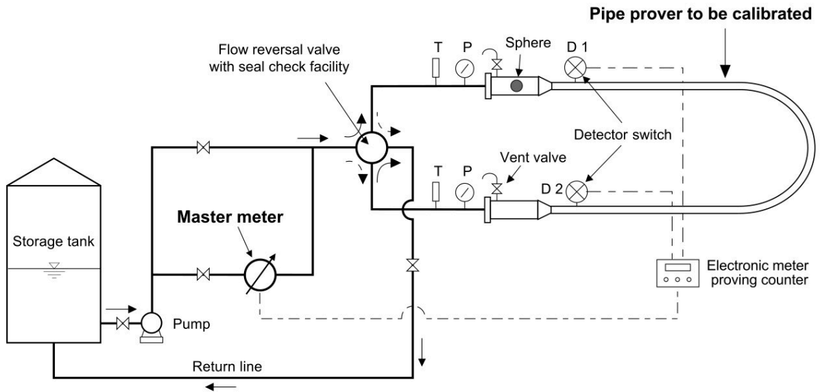
Figure A.9 — Calibration of a pipe prover (master meter method)
