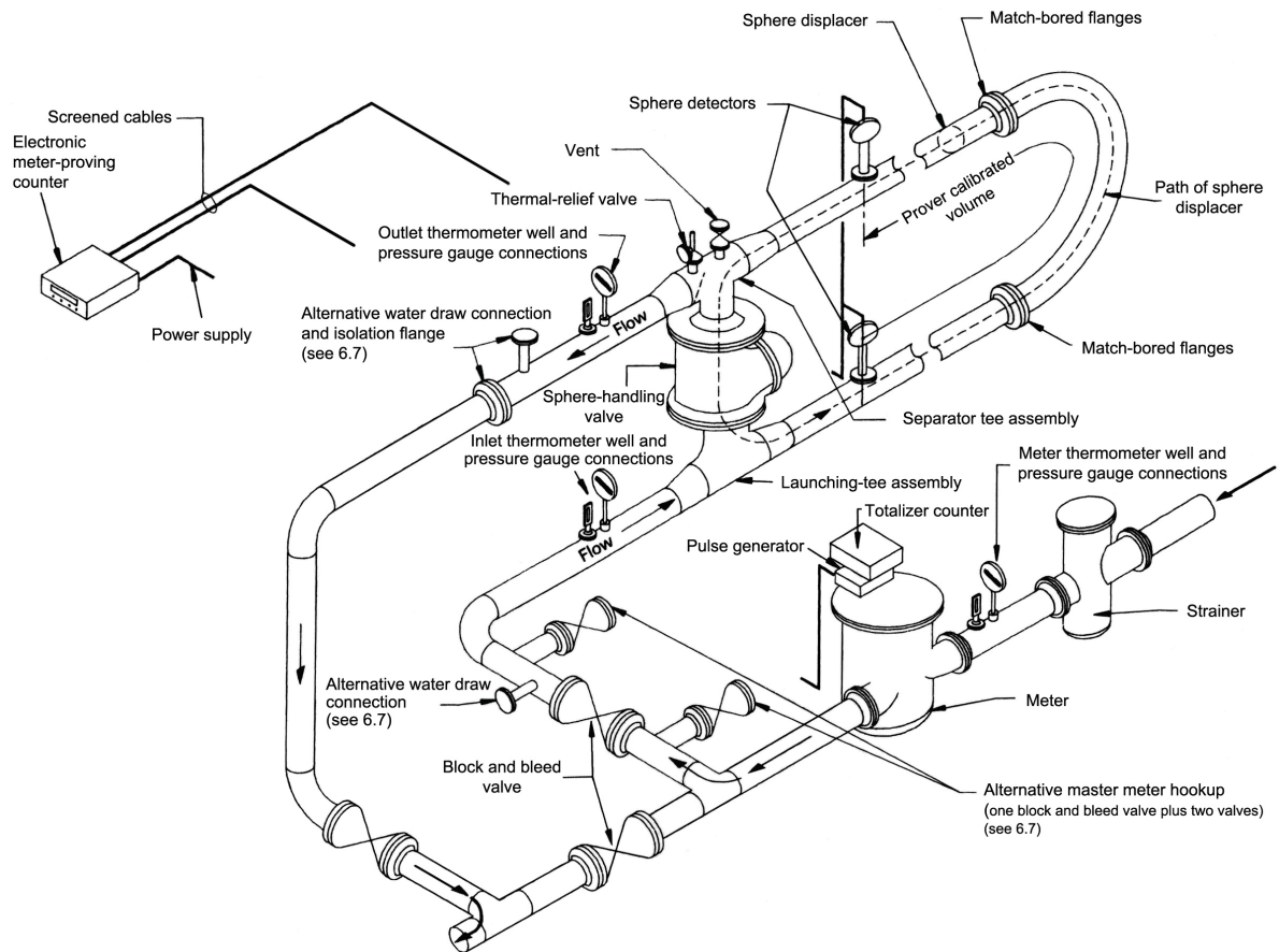
Figure A.1 — Typical uni-directional pipe prover (Extracted from ISO 7278-2:1988 2) )
