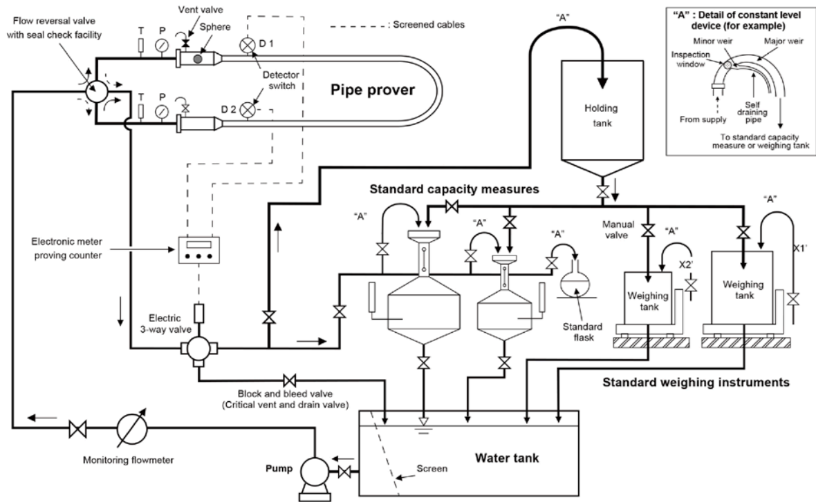
Figure A.7 — Calibration of pipe prover (water draw method)
