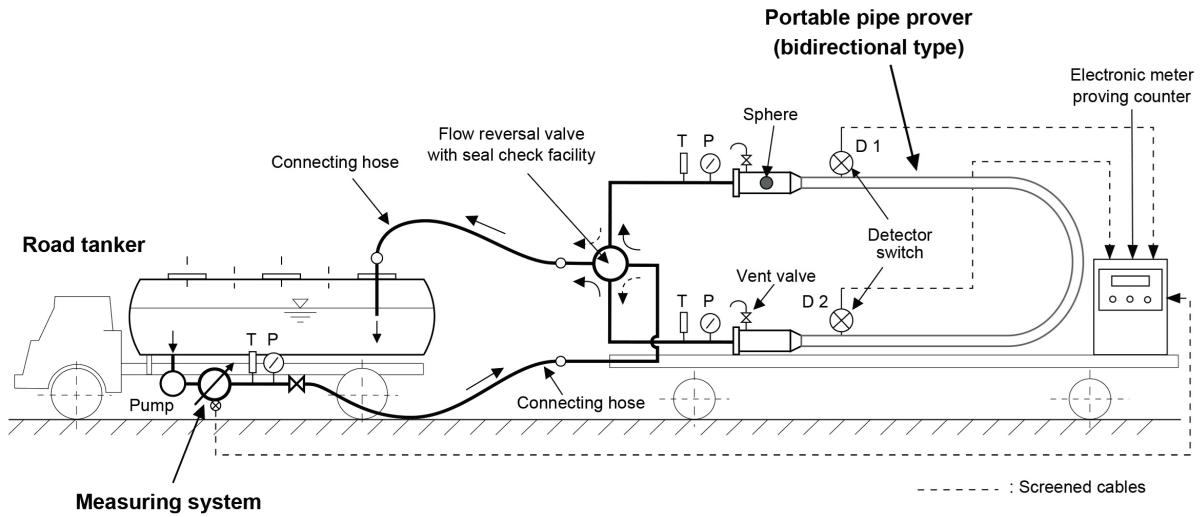
Figure A.11 — Verification of measuring systems on road tankers
