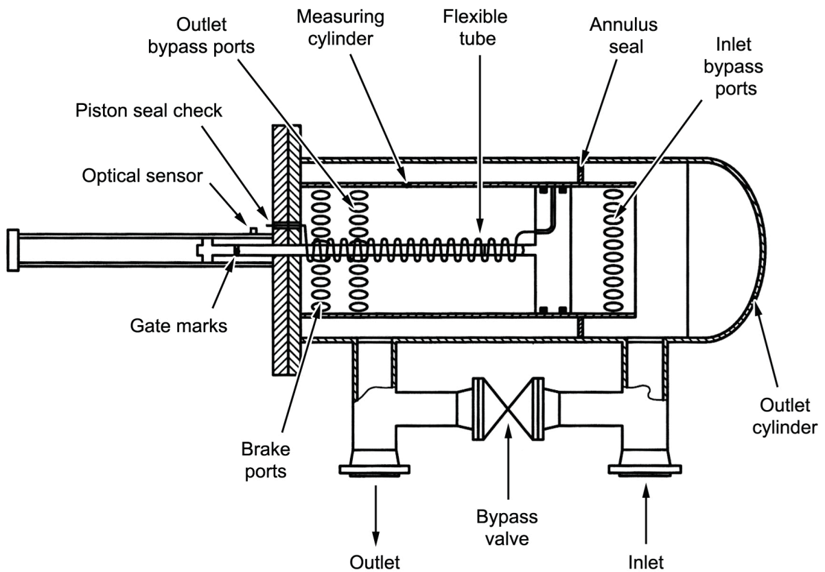
Figure A.5 — Typical small volume pipe prover with external valve (Extracted from ISO 7278-4:1999 2) )
