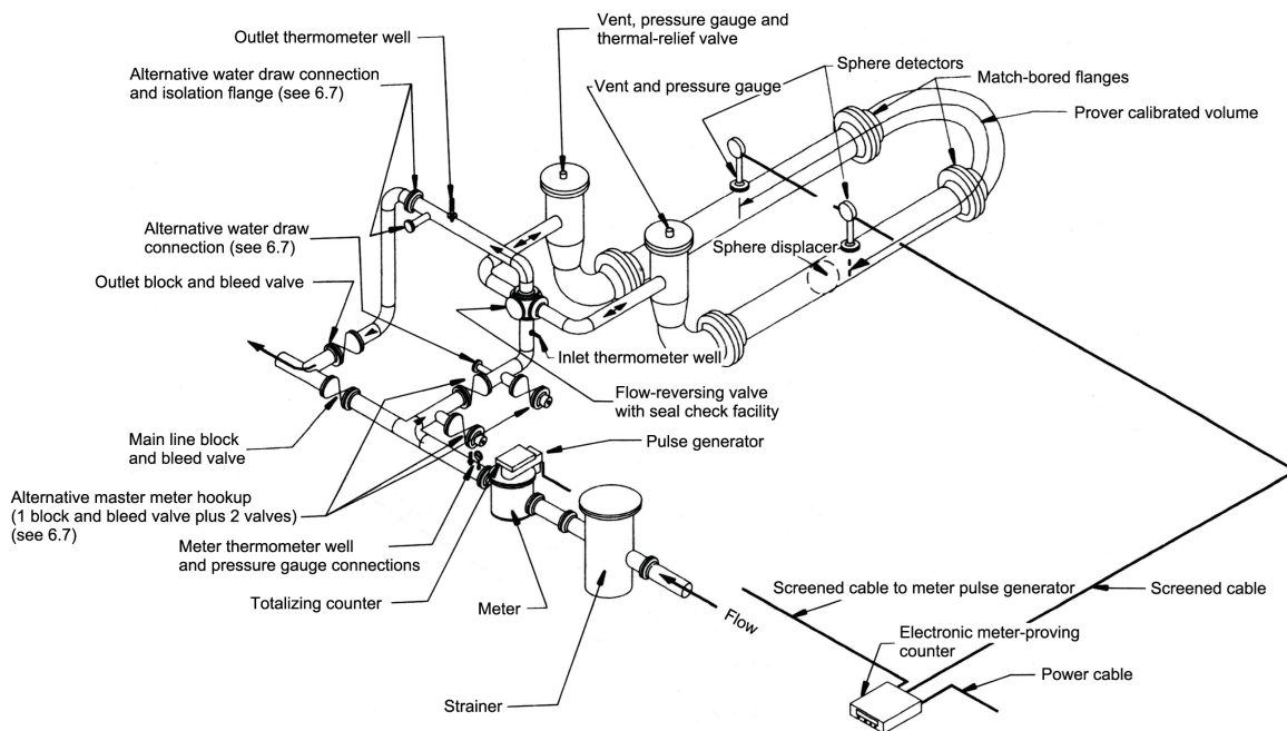
Figure A.3 — Typical bi-directional U-type pipe prover (Extracted from ISO 7278-2:1988 2) )
