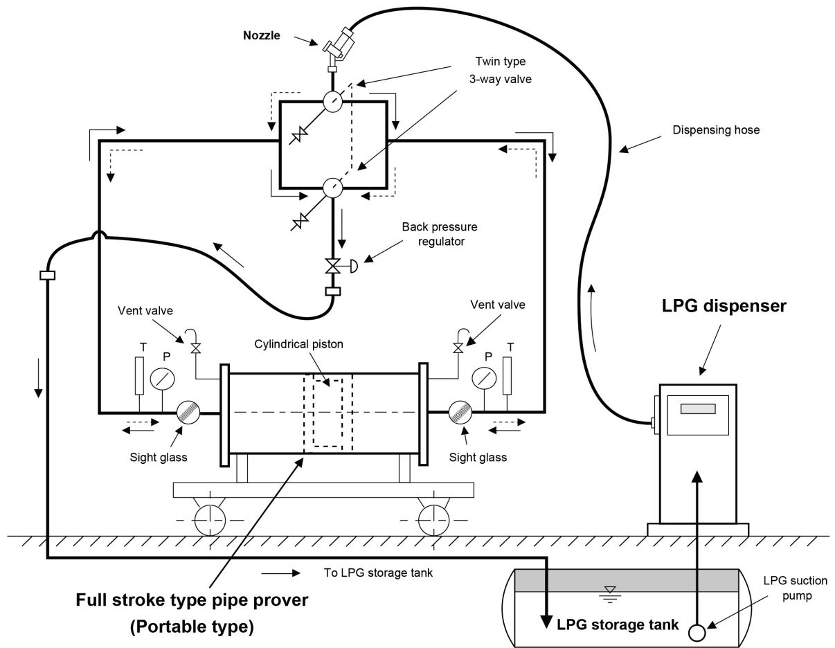
Figure A.13 — Verification of LPG dispensers
