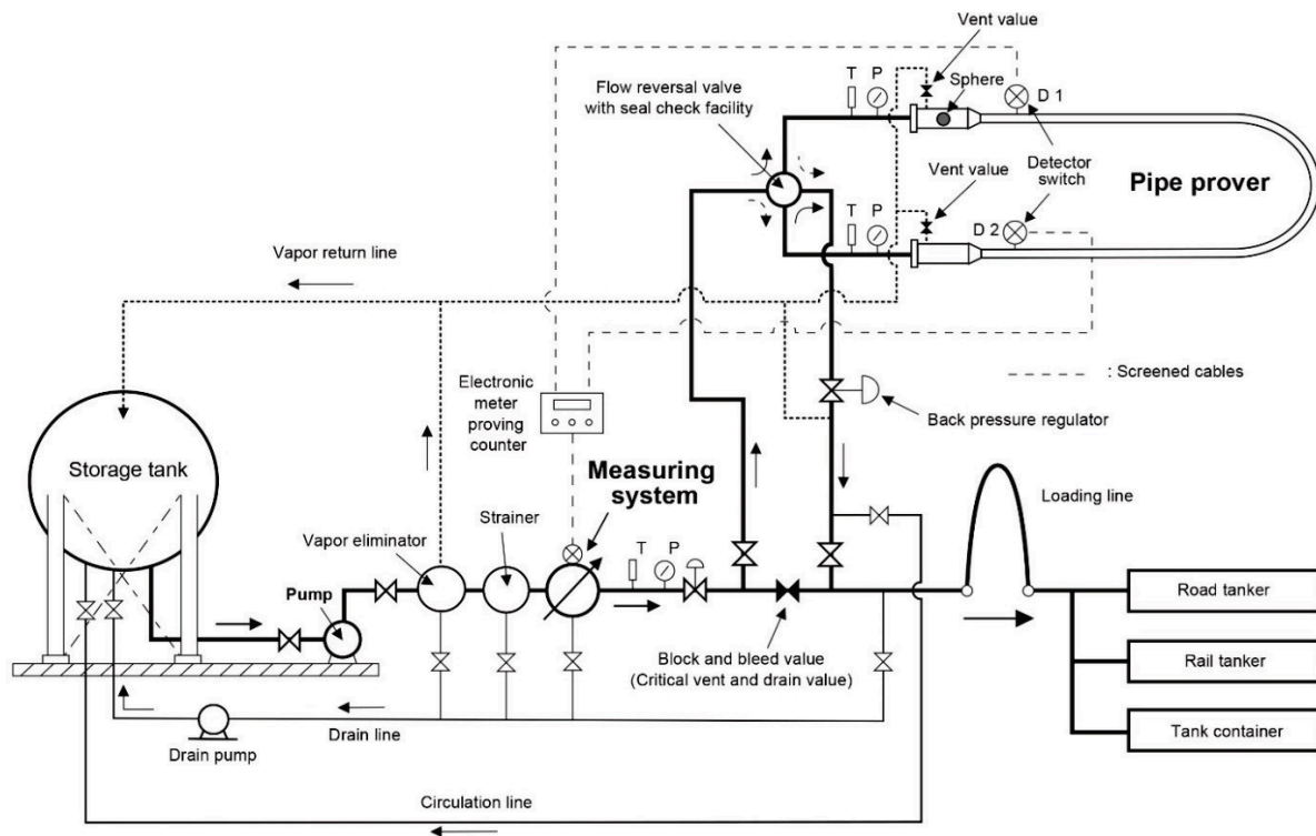
Figure A.12 — Verification of measuring systems for LPG under pressure
