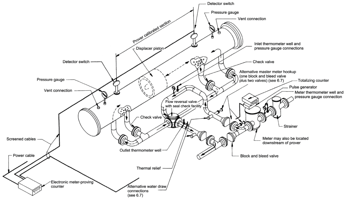
Figure A.2 — Typical bi-directional straight-type piston pipe prover (Extracted from ISO 7278-2:1988 2) )
