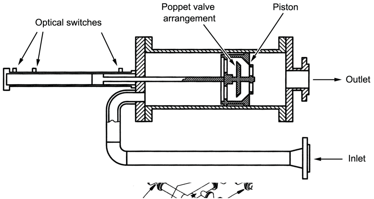
Figure A.4 — Typical small volume pipe prover with internal valve (Extracted from ISO 7278-4:1999 2) )
