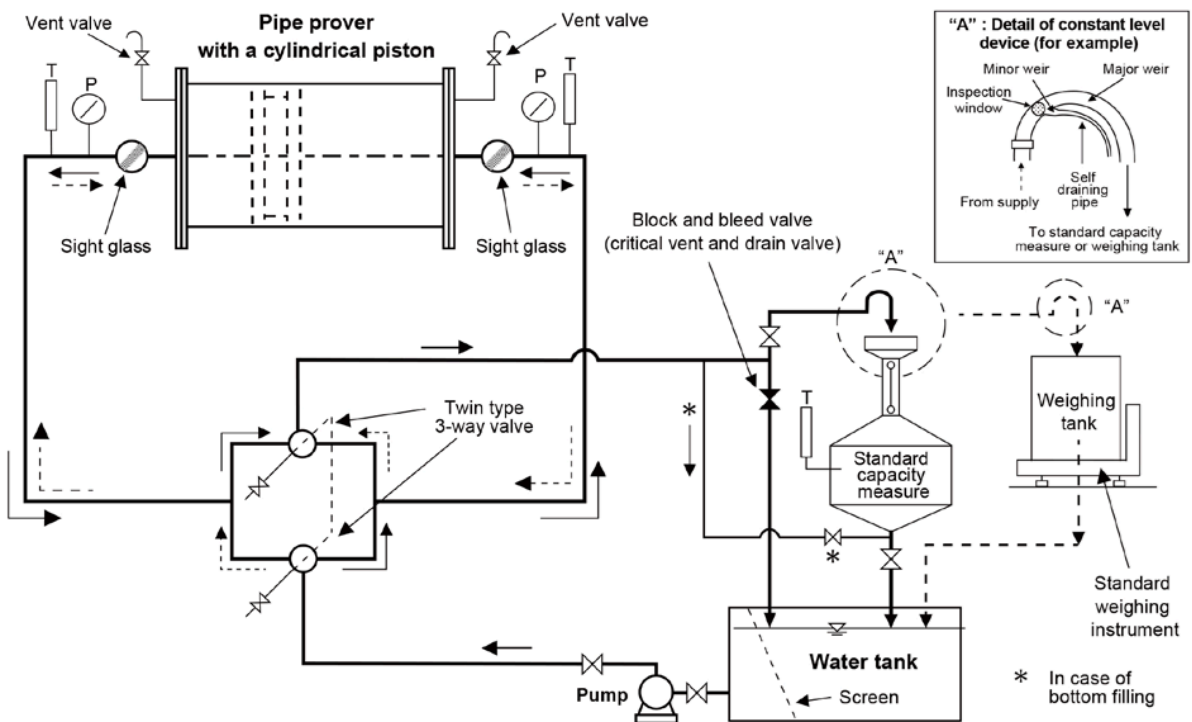
Figure A.8 — Calibration of full stroke type pipe prover (water draw method)
