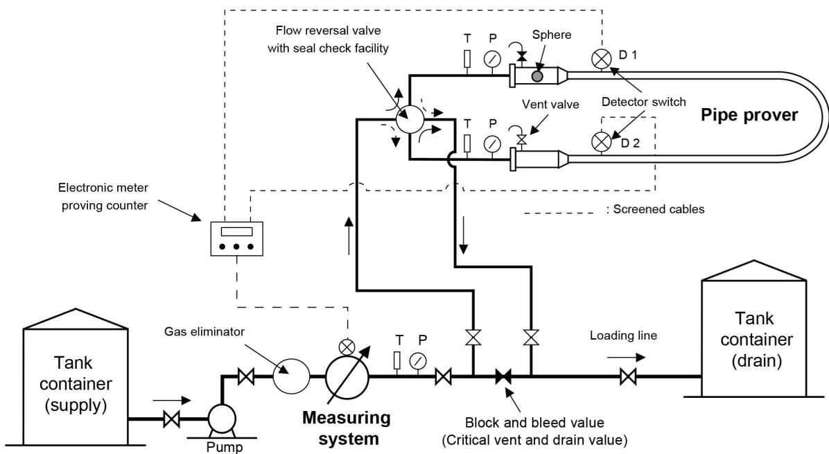
Figure A.10 — Verification of measuring systems for tank containers connected with pipelines
