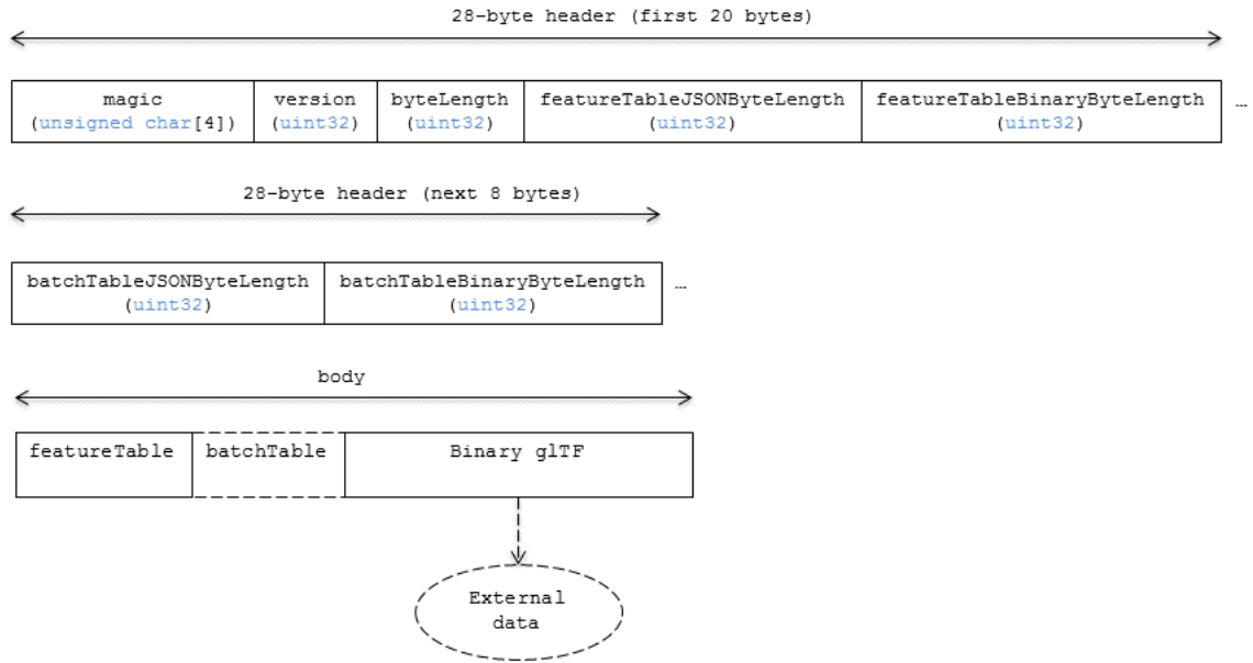
Figure 24 – Batched 3D Model layout
