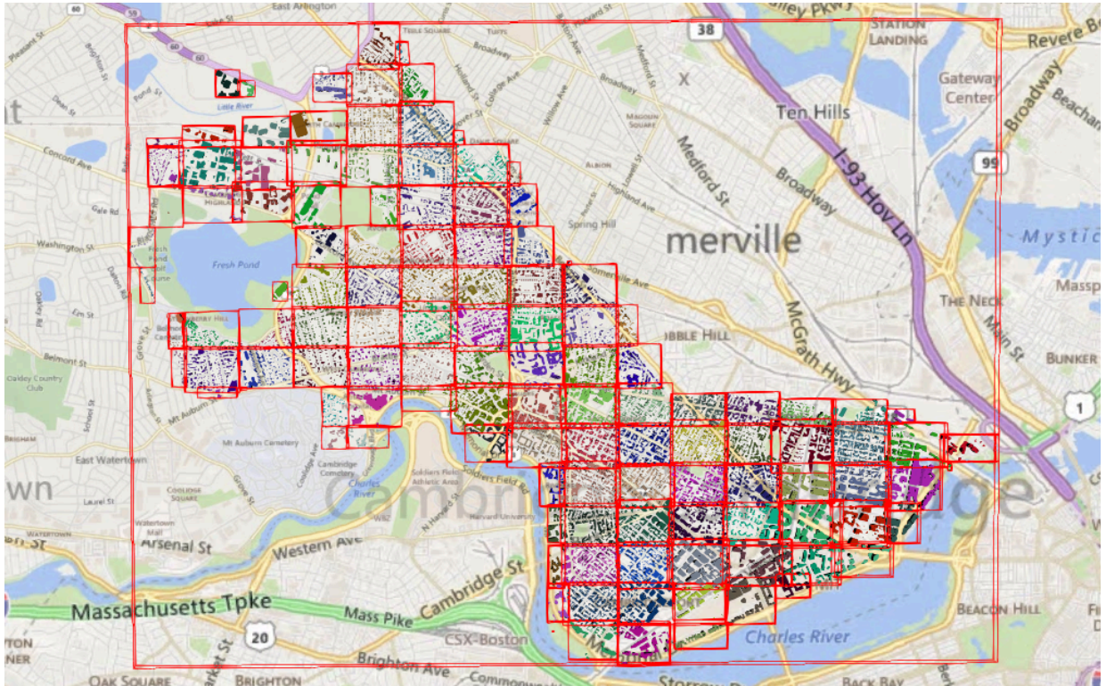
Figure 19 – A tileset with an overlapping grid spatial data structure
