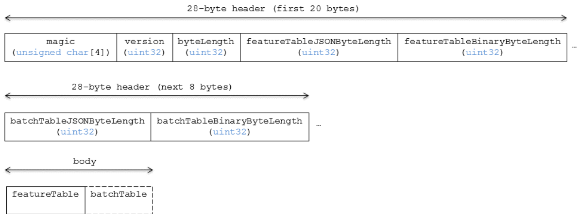
Figure 29 – Point Cloud layout
