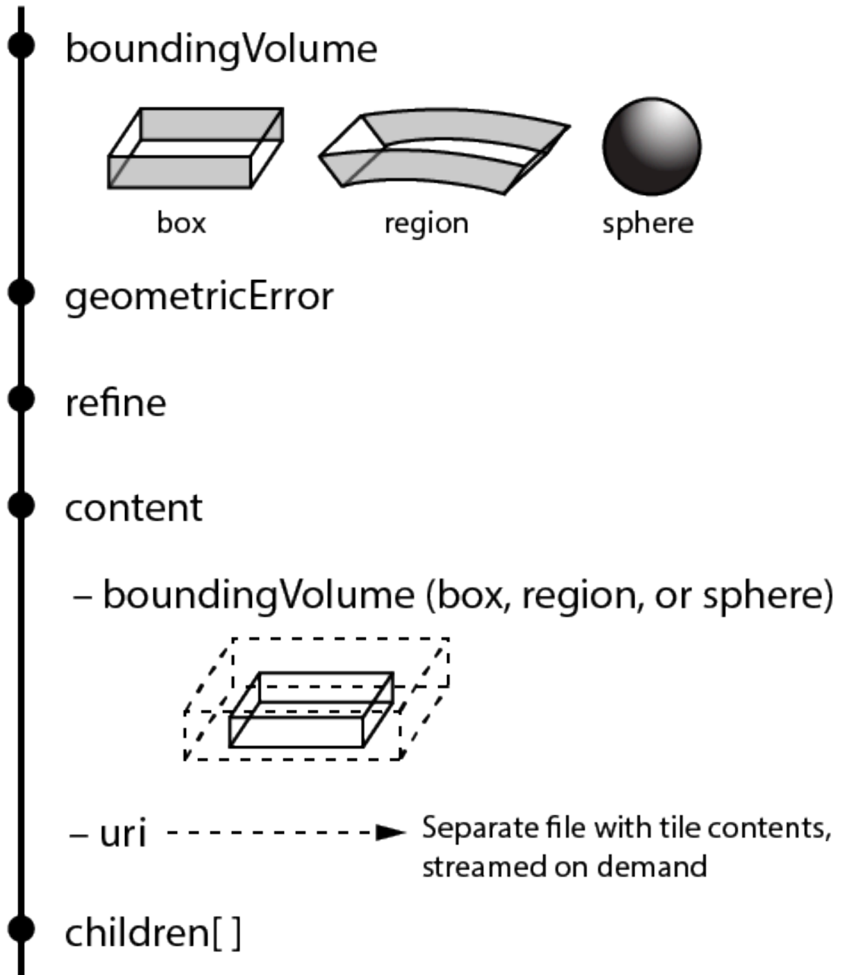
Figure 13 – Tile JSON properties
