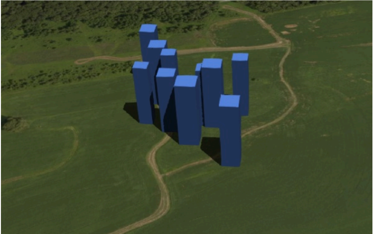
Figure 4 – A parent tile with additive refinement
