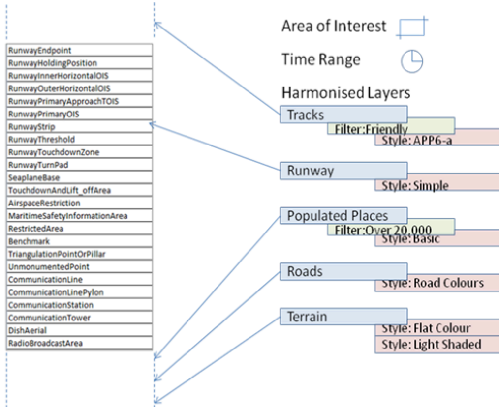
Figure 5 – Structure of OWS Context Document
