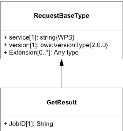
Figure 23 – GetResult request UML class diagram
