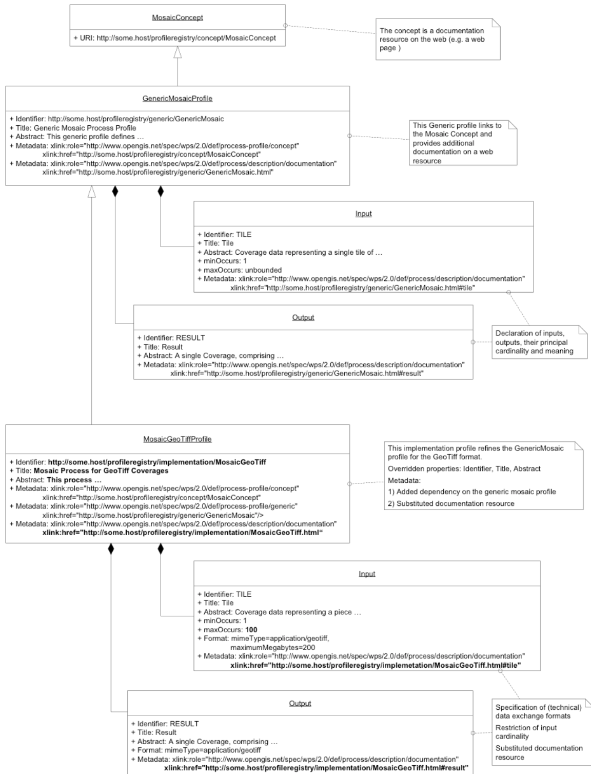
Figure B.3 – Profile inheritance example for a mosaic process
