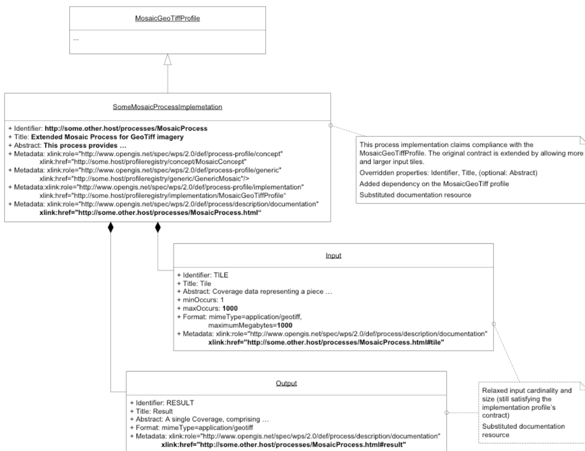
Figure B.4 – Profile inheritance example for a mosaic process, extension by an implementation
