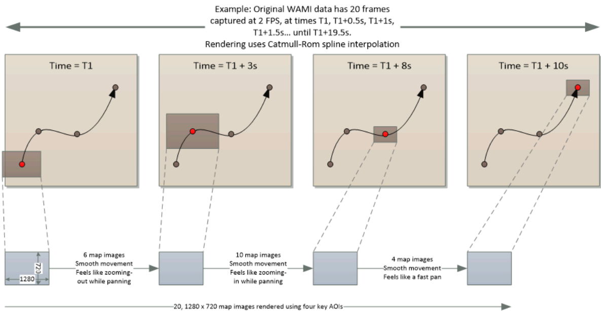
Figure 14 – Key-frame animation using GetPathMap and GetPathMapVideo
