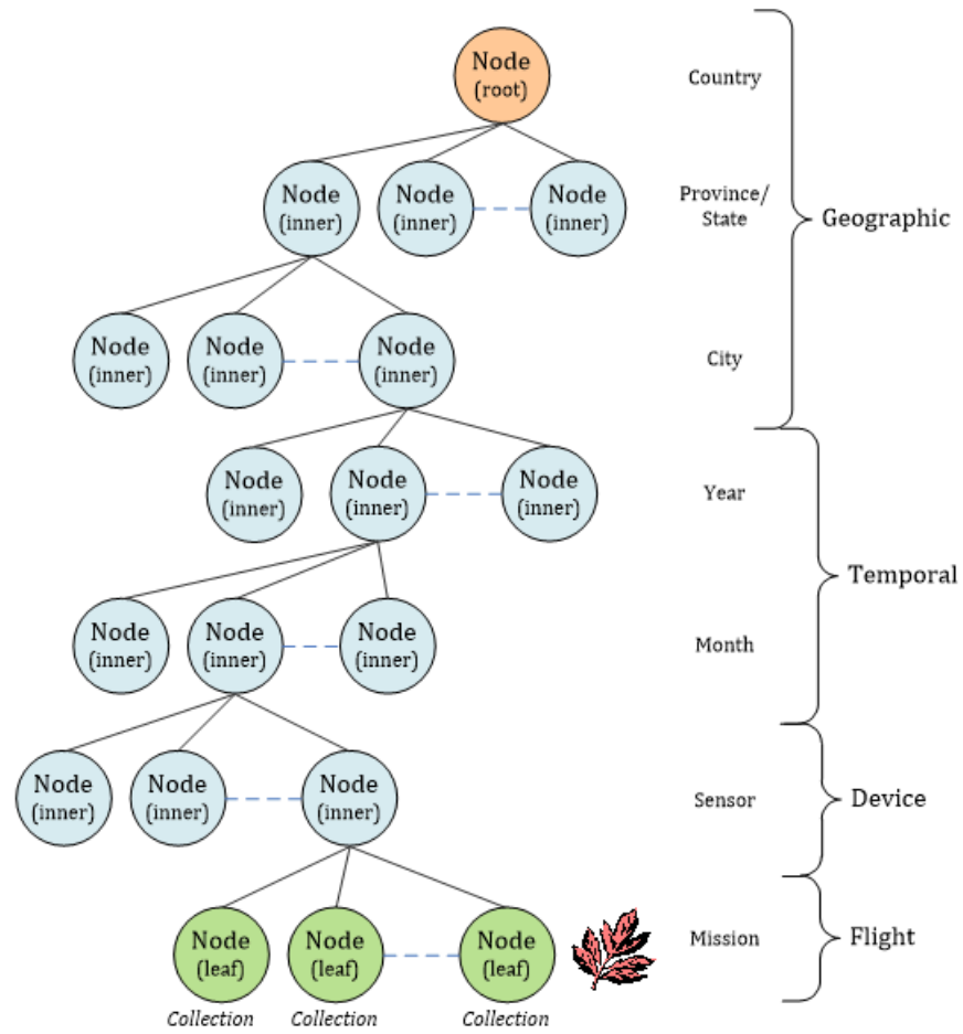
Figure 9 – Collection tree served by a collection service
