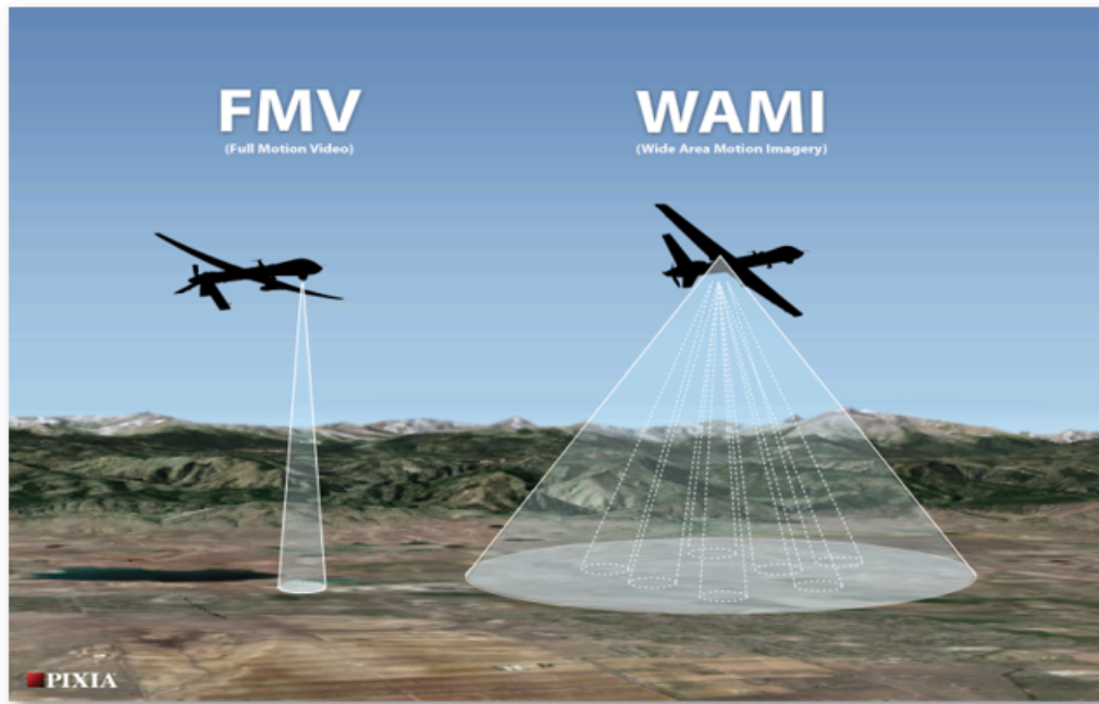
Figure 6 – FMV vs. WAMI coverage
