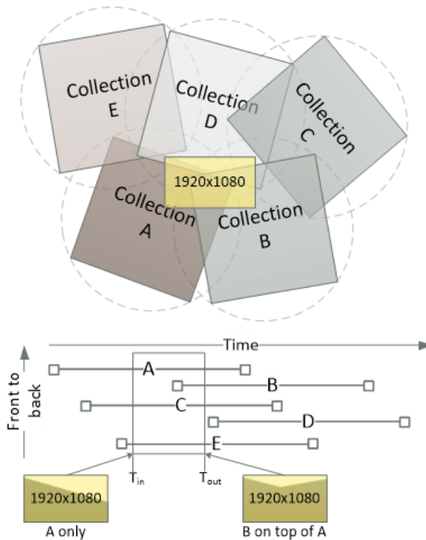
Figure 13 – Spatial overlap can change over time
