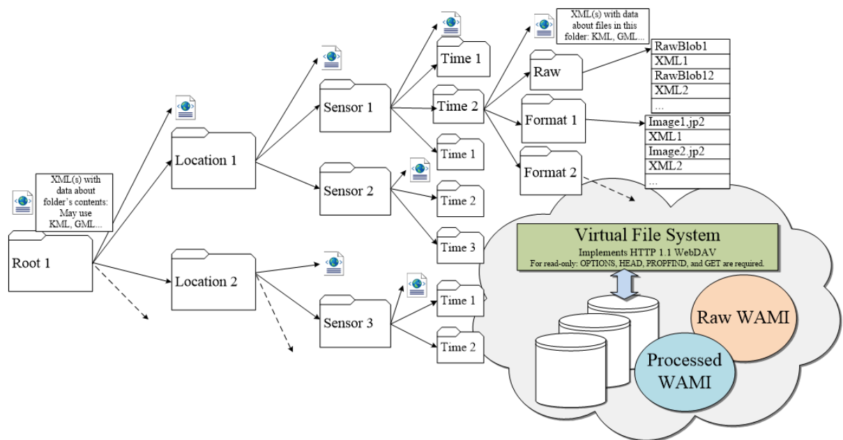
Figure 8 – Virtual file system using HTTP 1.1 WebDAV
