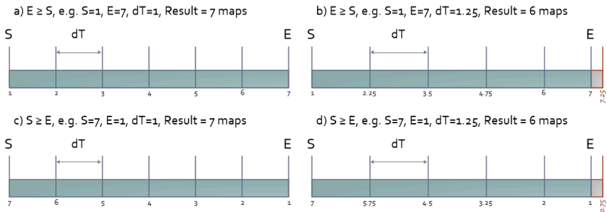
Figure 11 – Consistently resolve temporal ambiguity
