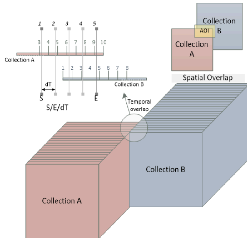
Figure 12 – Consistently resolve spatiotemporal ambiguity
