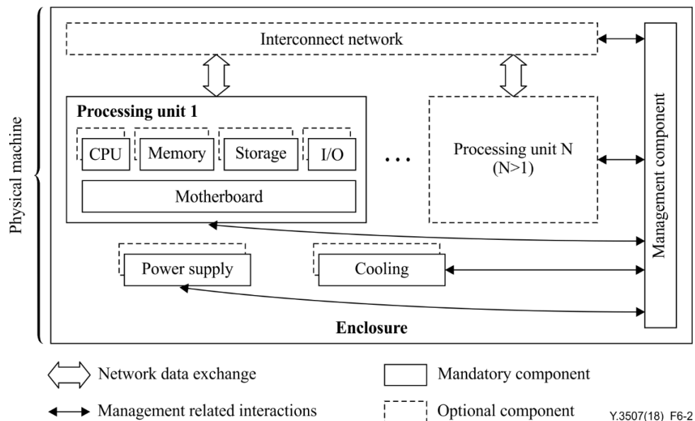
Figure 2 — Overview of the physical machine
