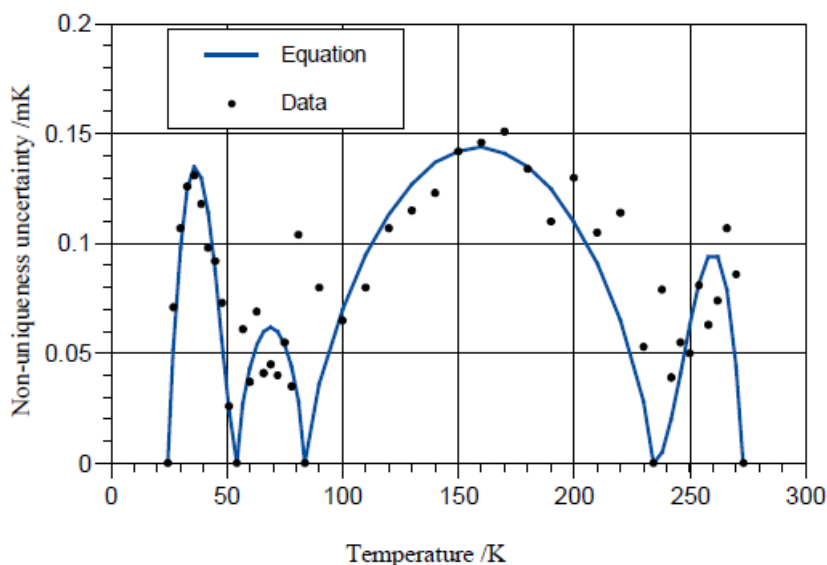
Figure 10 — The measured uncertainty (standard deviation) due to Type 3 non-uniqueness in the range 24.556 1 K to 273.16 K (from the data of Hill and Steele (2003) ) and the functional approximation of Table 6.
