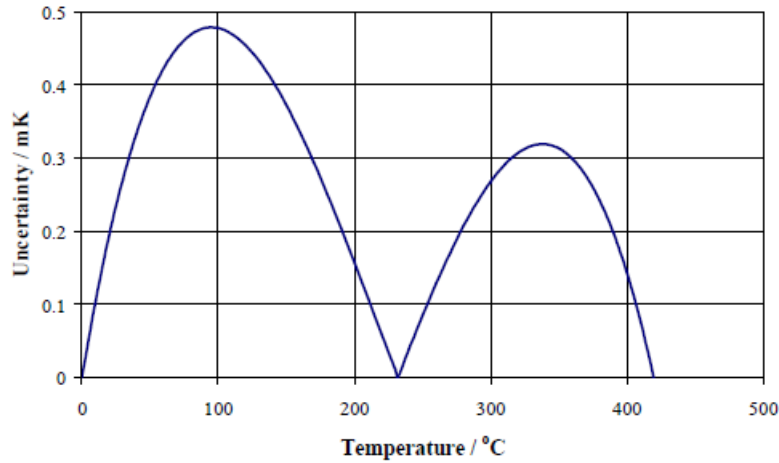
Figure 7 — Standard deviation of the sub-range inconsistency over the range 0 °C to 420 °C for a group of 50 SPRTs, from White and Strouse (2009) . The maxima occur at 93.15 °C ( W = 1.366\,227 ) and 336.57 °C ( W = 2.274\,97 ). (1)
