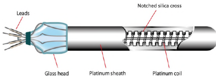
Figure 1 — Schematic diagram of a typical 25 Ω capsule-type SPRT. The sensing element is formed from fine, \sim 0.07 mm diameter, coiled platinum wire supported on a notched high-purity silica cross. The four lead wires are welded to the sensing element, two at each end, and pass through the glass seal. The platinum sheath is about 5 mm in diameter and 50 mm long. (Illustration published on courtesy from FLUKE®)
