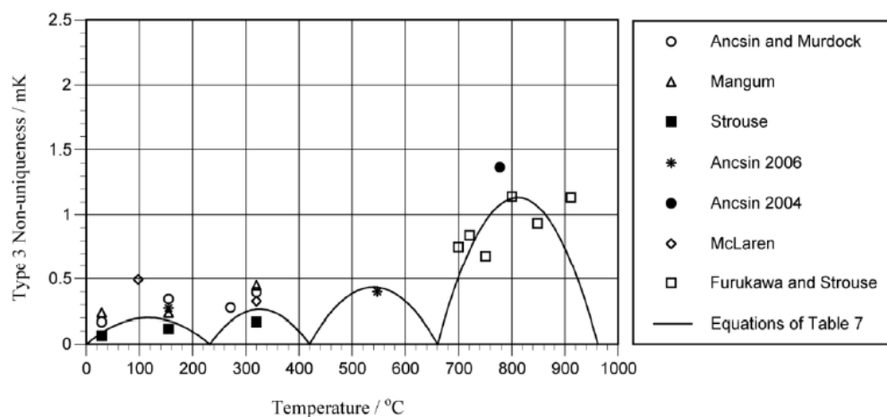
Figure 11 — Summary of available data on Type 3 non-uniqueness of ITS-90 above 0 °C. The data of Mangum and McLaren are from Hill and Woods (1992) . The solid line shows the curves defined by the polynomials of Table 7.
