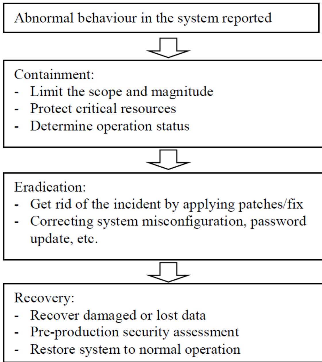
Figure 4 – Major Stages in Security Incident Response
